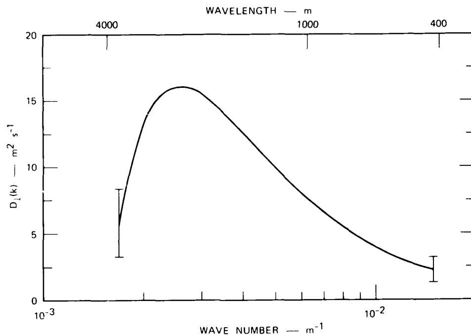
Figure IV.A.7. Empirically derived diffusion coefficient.
