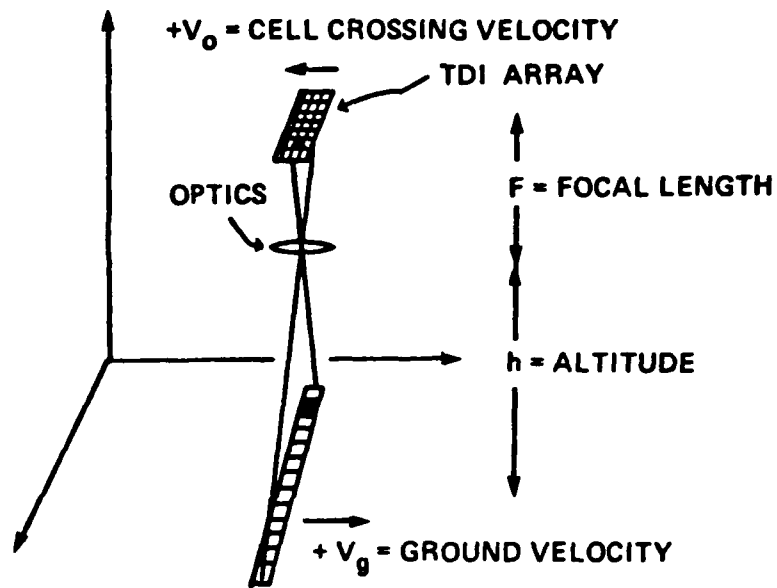
Figure 11. Push-Broom Scanned Array.
