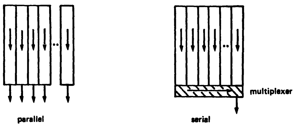
Figure 2. Readout of CCD Unit Cells [6].
