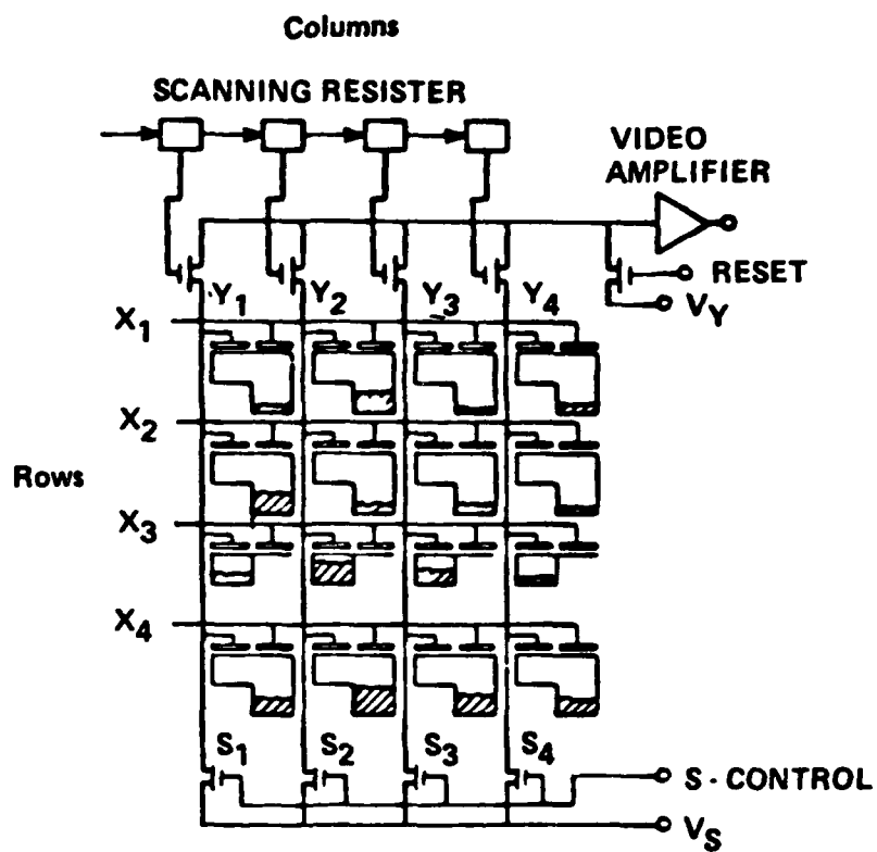
Figure 4. Readout of a matrix of CID unit cells [4].
