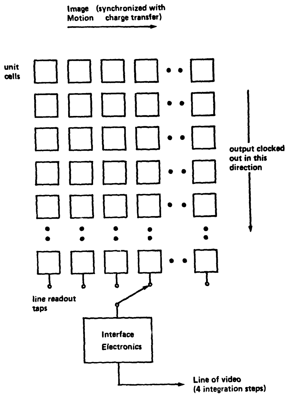
Figure 7. Linear TDI array.
