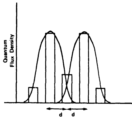
Figure 13b. Two points resolved at Nyquist rate.
