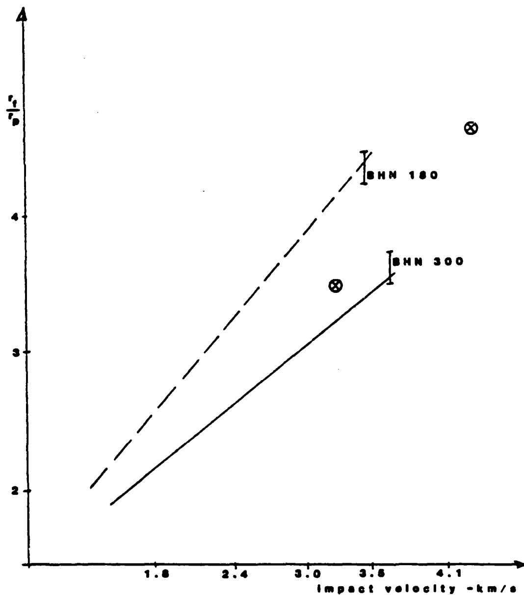
Figure 21. The Normalized Cavity Dimension Variation with Respect to Impact Velocity and Target Strength for Tungsten Rods and Steel Targets.
