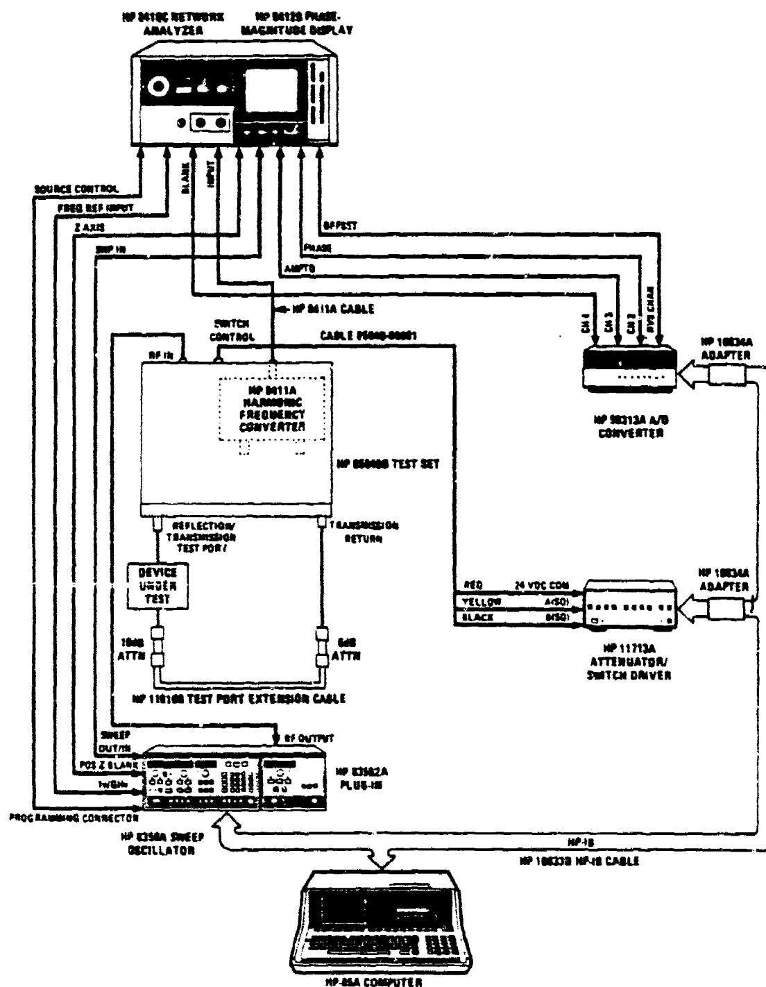
Figure 7. Signal Flow When Measuring S-parameters. Schematic Taken from Hewlett-Packard Manual for the 85040B Test Set, pp. 2-8, May 1982.
