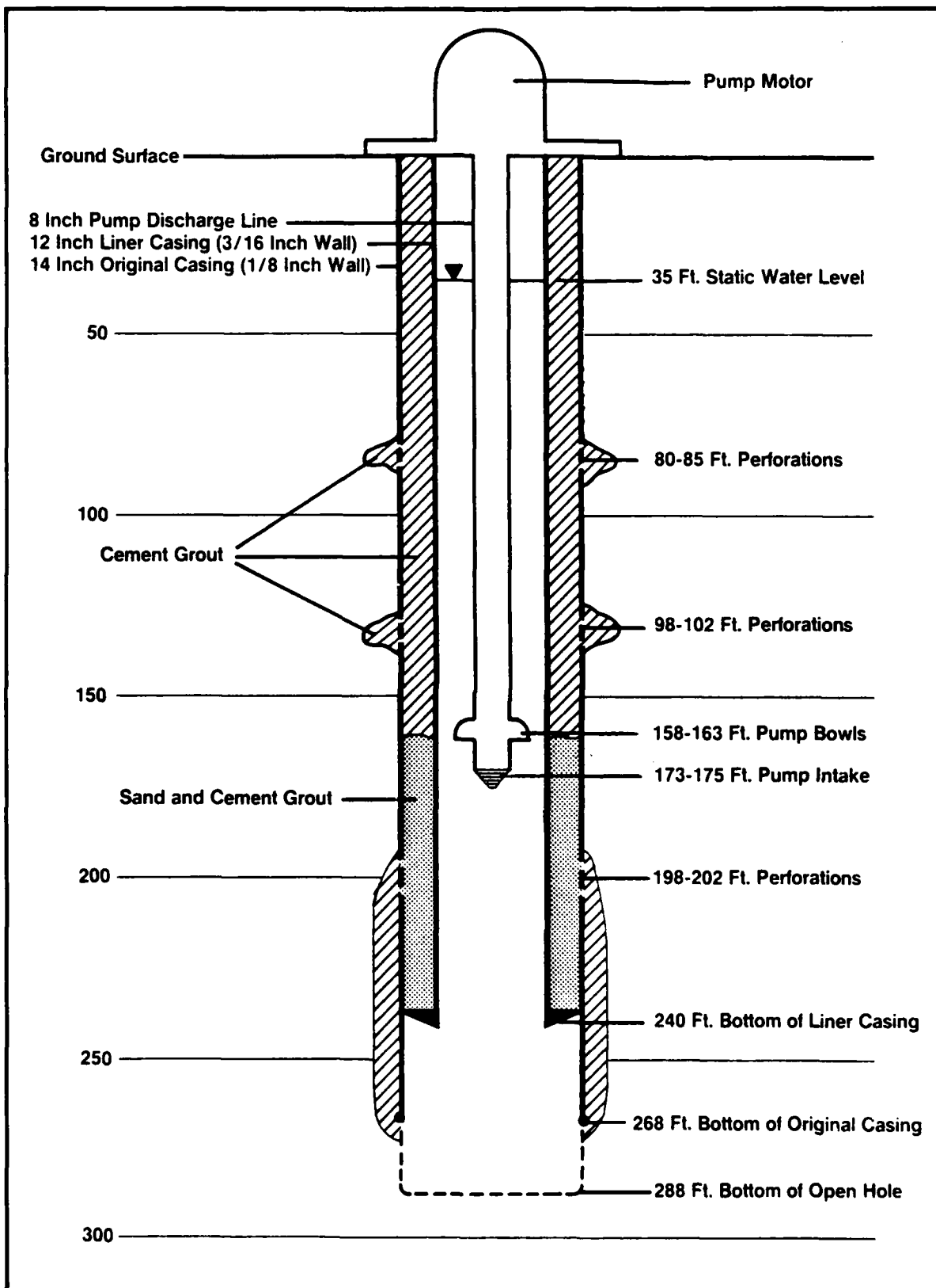
FIGURE 3-22 SCHEMATIC OF REHABILITATED BASE PRODUCTION WELL 3
