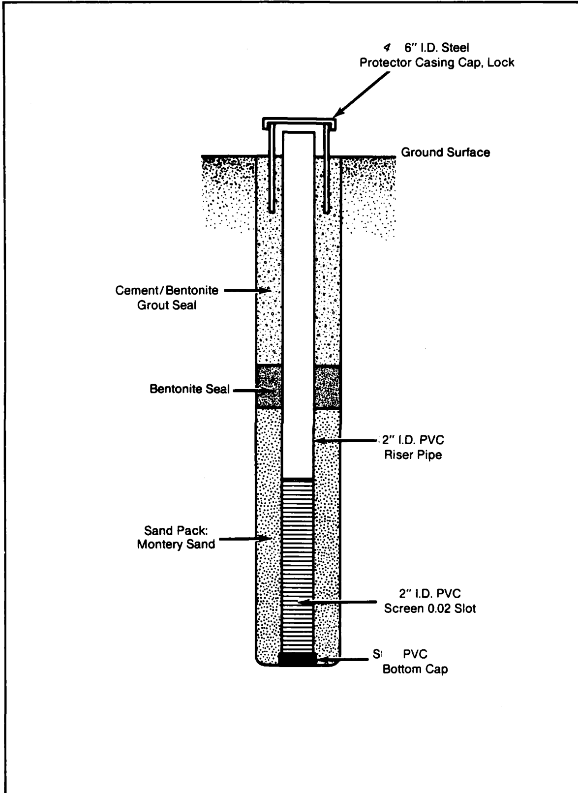
FIGURE 3-14. TYPICAL LYSIMETER CONSTRUCTION
