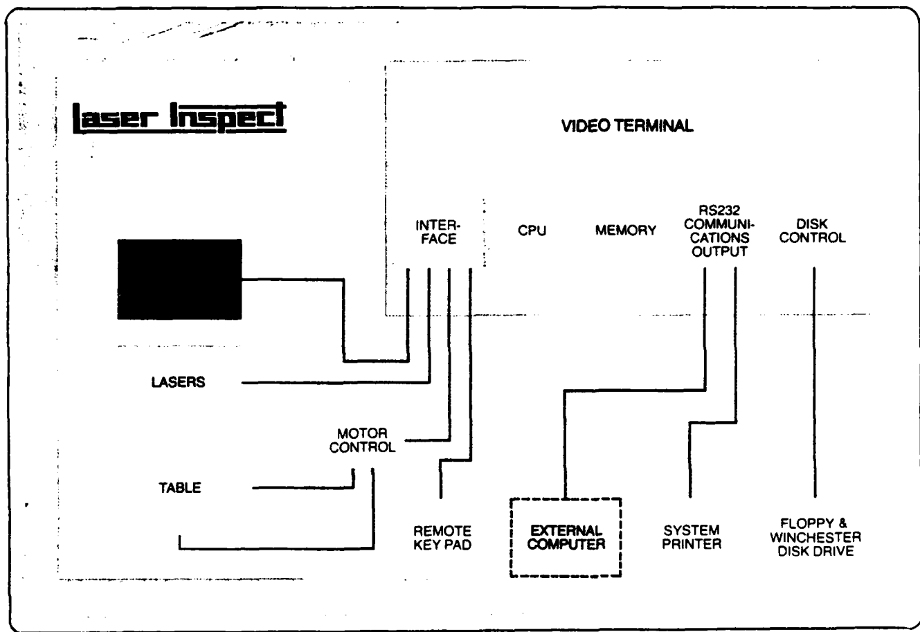
Figure 11. Electronics block diagram of the Li/6000.
