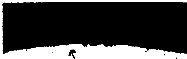
Figure 4 - INTERMETALLIC BETWEEN COPPER LEAD AND TIN PLATING
