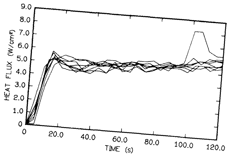
FIGURE 2.3. MEASURED DOORWAY HEAT FLUX VS TIME (LOWER FLUXMETER; TESTS 104-111).
