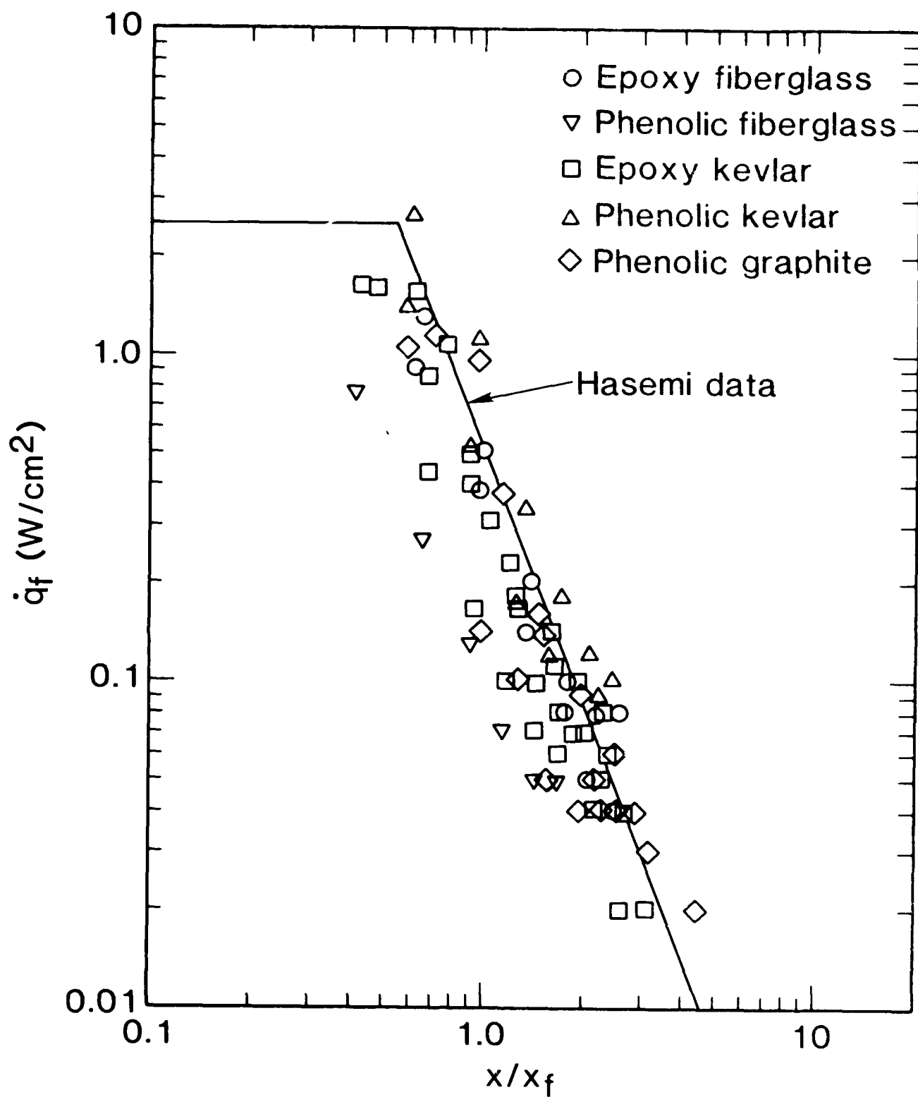
FIGURE 3.16. WALL HEAT FLUX DISTRIBUTION FOR FIVE AIRCRAFT PANELS AT 3.8 W/cm 2 EXTERNAL IRRADIANCE.
