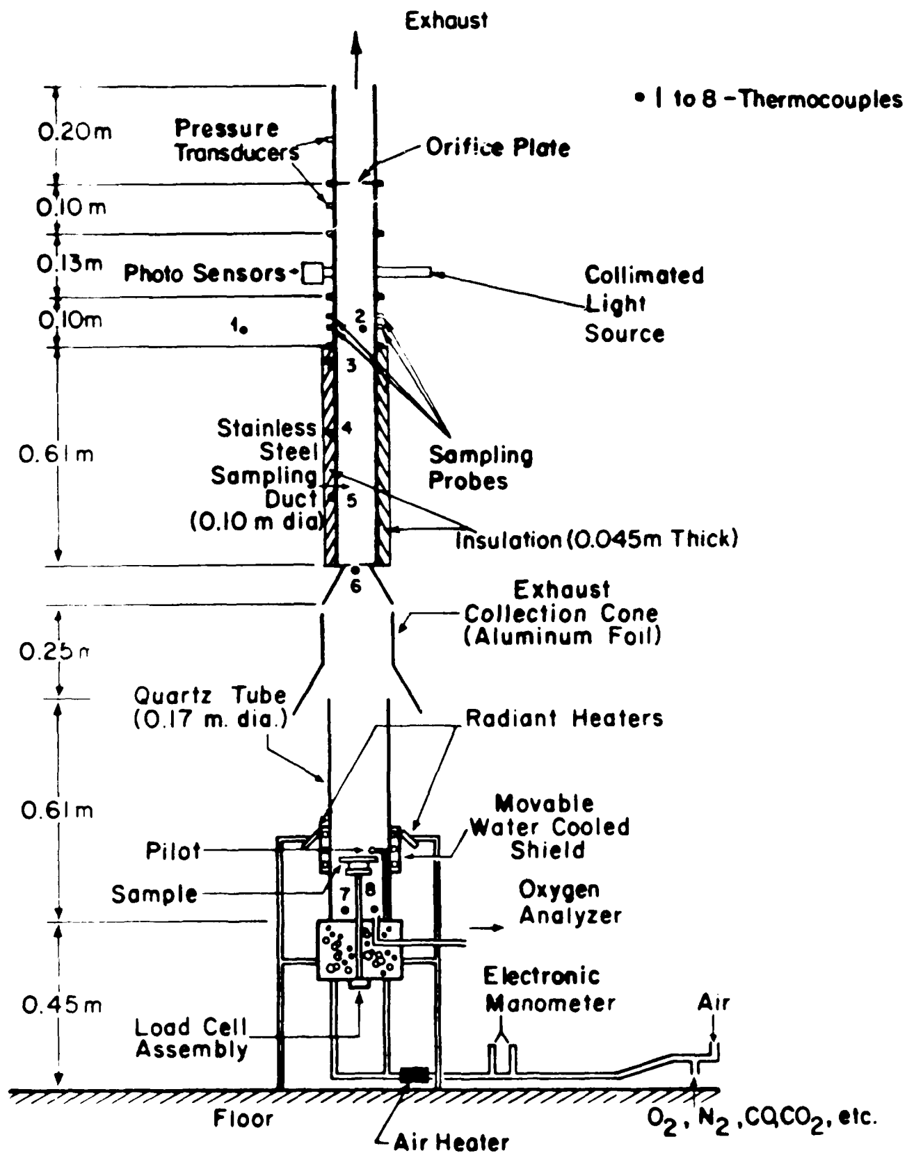
FIGURE 5.1. EXPERIMENTAL APPARATUS
