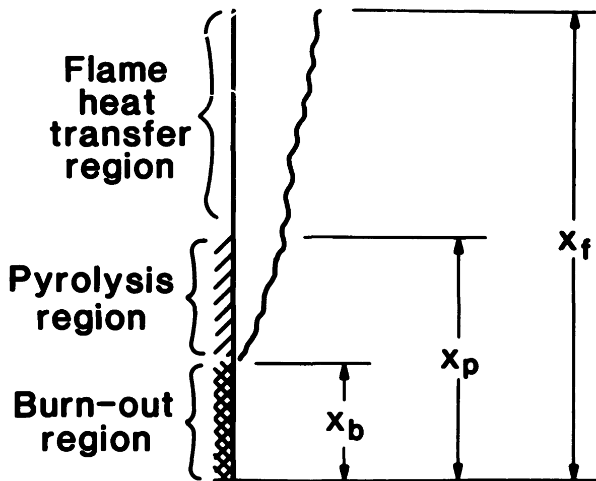
FIGURE 3.10. SCHEMATIC OF FLAME SPREAD PROBLEM.
