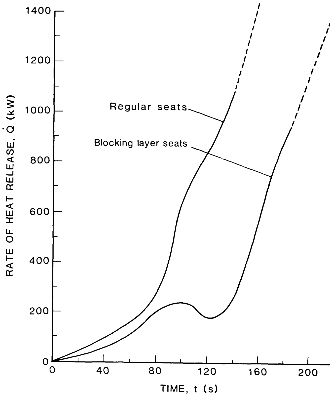
FIGURE 2.16. ESTIMATE FOR \dot{Q}_{\text{seat}} FOR ARRAYS OF POLYURETHANE SEATS WITH AND WITHOUT BLOCKING LAYERS [13] (— — — — — EXTRAPOLATED FROM CURVES OF [13]).
