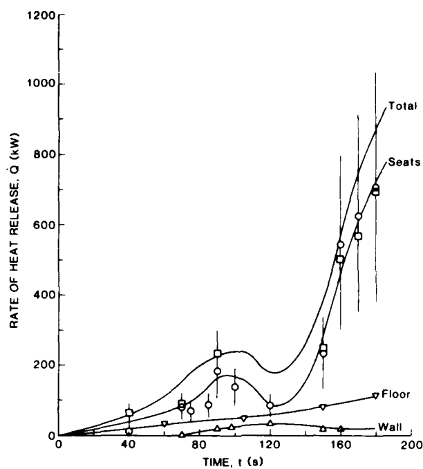
FIGURE 1.9. ESTIMATES OF HEAT RELEASE RATES DURING TEST 34 (VONAR-3 SEATS). SYMBOLS: ○, ▽, Δ - BASED ON AREA-OF-INVOLVEMENT AND CALORIMETER HEAT RELEASE DATA: □ - BASED ON FLAME HEIGHT DATA.
