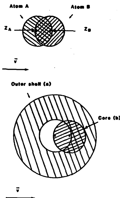
Fig. 8. Approximate correspondence between (top) A-B atom-atom collision at relative velocity \nu and (bottom) coherent relative motion of outer-shell electrons (a) with respect to core (b). For simplicity, the electrons in the bottom half of the figure are depicted as undistorted, mutually displaced charge distributions moving with relative velocity \nu . The nuclear charges of the projectile and target systems, Z_A and Z_B , respectively, are denoted in the atom-atom collisions.
