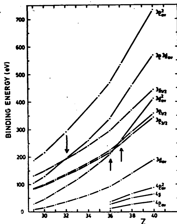
FIG. 8. Atomic, relativistic \Delta SCF single- and double-hole levels for _{29}\text{Cu} to _{40}\text{Zr} . The energies were obtained from Ref. 48 and the figure has been adapted from Fig. 17 of Ref. 43 appearing on p. 28. The arrows indicate the locations of near degeneracies between single- and double-vacancy states. Figure reprinted by permission.
