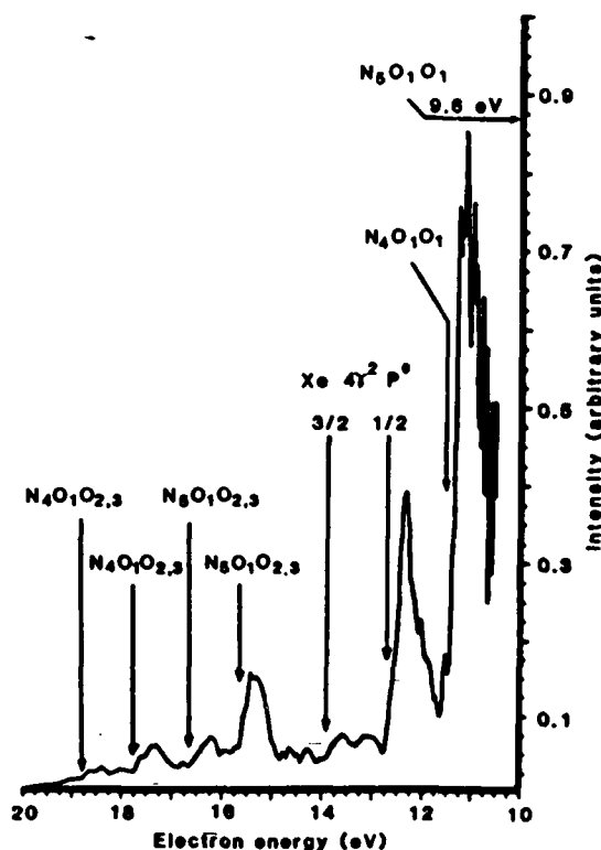
Fig. 7. Prominent transitions observed in the electron spectrum of Xe irradiated at 193 nm and approximately 10^{15} W/cm 2 . Both continuum-continuum ( 4\gamma \rightarrow Xe_{3/2}^+, Xe_{1/2}^+ ) and tentatively assigned Auger ( N_{6,00} ) features are apparent. The splittings between the three N_6-N_5 pairs, two of which are shown by horizontal arrows, have the common value of about 2 eV, which is the known 4d_{3/2} to 4d_{5/2} separation in Xe. The vertical arrows indicate the high-energy edges of the observed features that represent the true energies of the lines.
