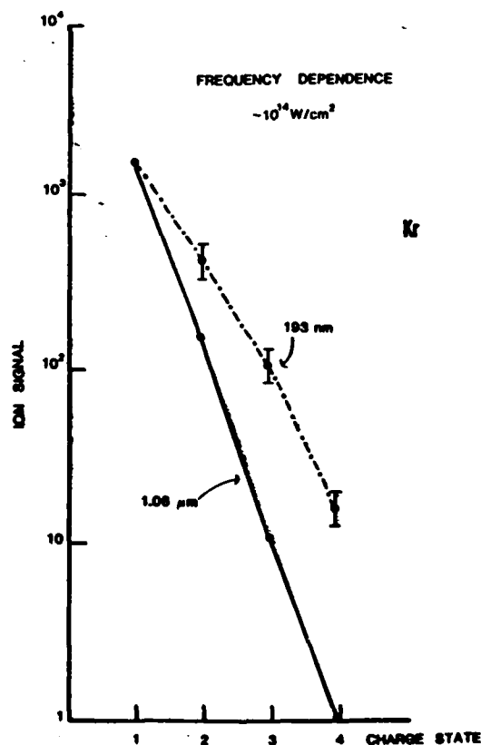
FIG. 6. Comparison of charge-state spectra observed for krypton at an intensity of \sim 10^{14} W/cm 2 at 1.06 \mu\text{m} and 193 nm. The data shown for 1.06 \mu\text{m} irradiation is taken from Ref. 19.
