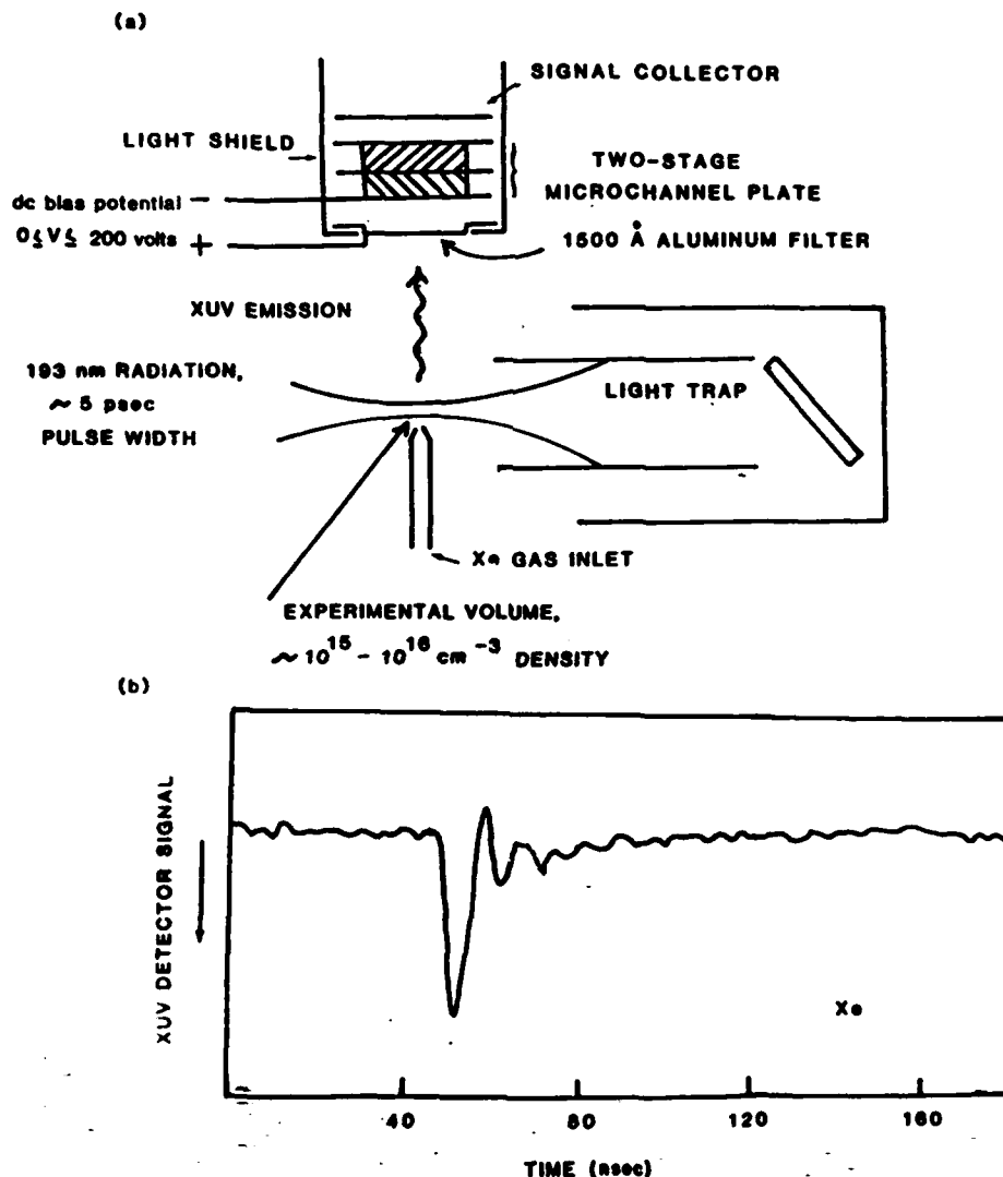
FIG. 10. (a) Experimental arrangement used to detect xuv radiation from highly excited atoms excited by 193-nm radiation at an intensity of \sim 10^{16} – 10^{17} W/cm 2 . (b) xuv signal observed from xenon in the 10–100 eV range with \sim 100 -V bias between the aluminum filter and the microchannel plate; some ringing of the detector circuit is evident.
