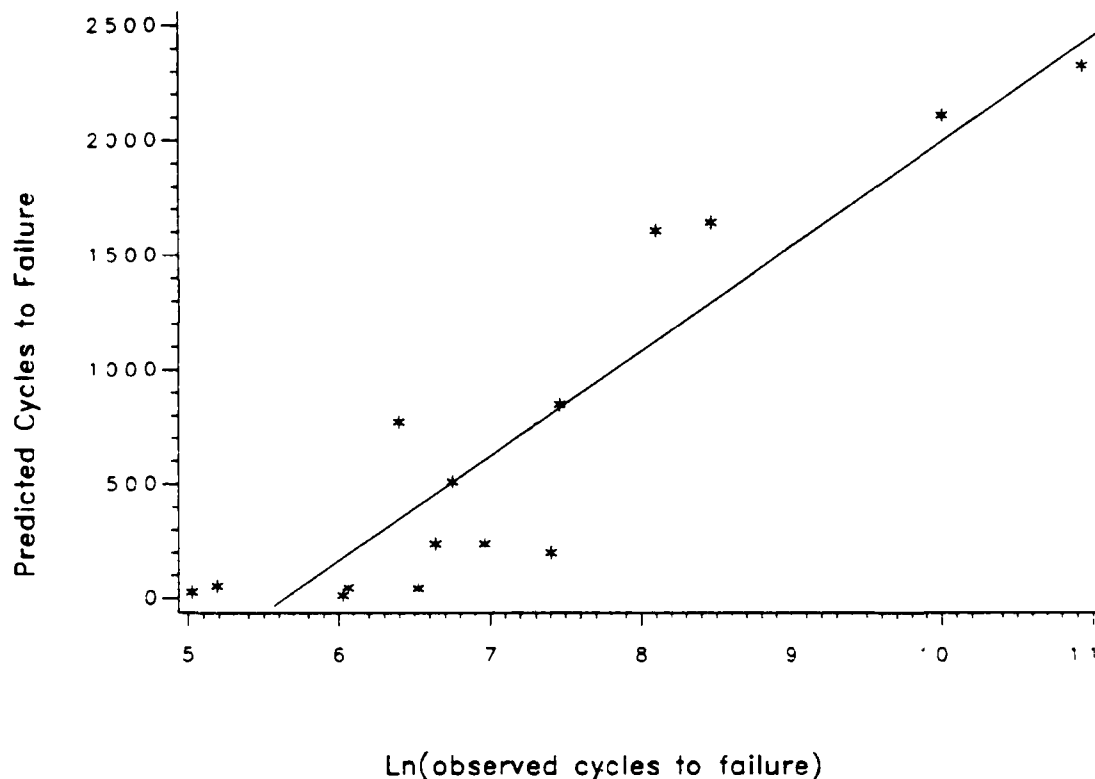
Figure 32. Prediction of failure cycle from static test.
