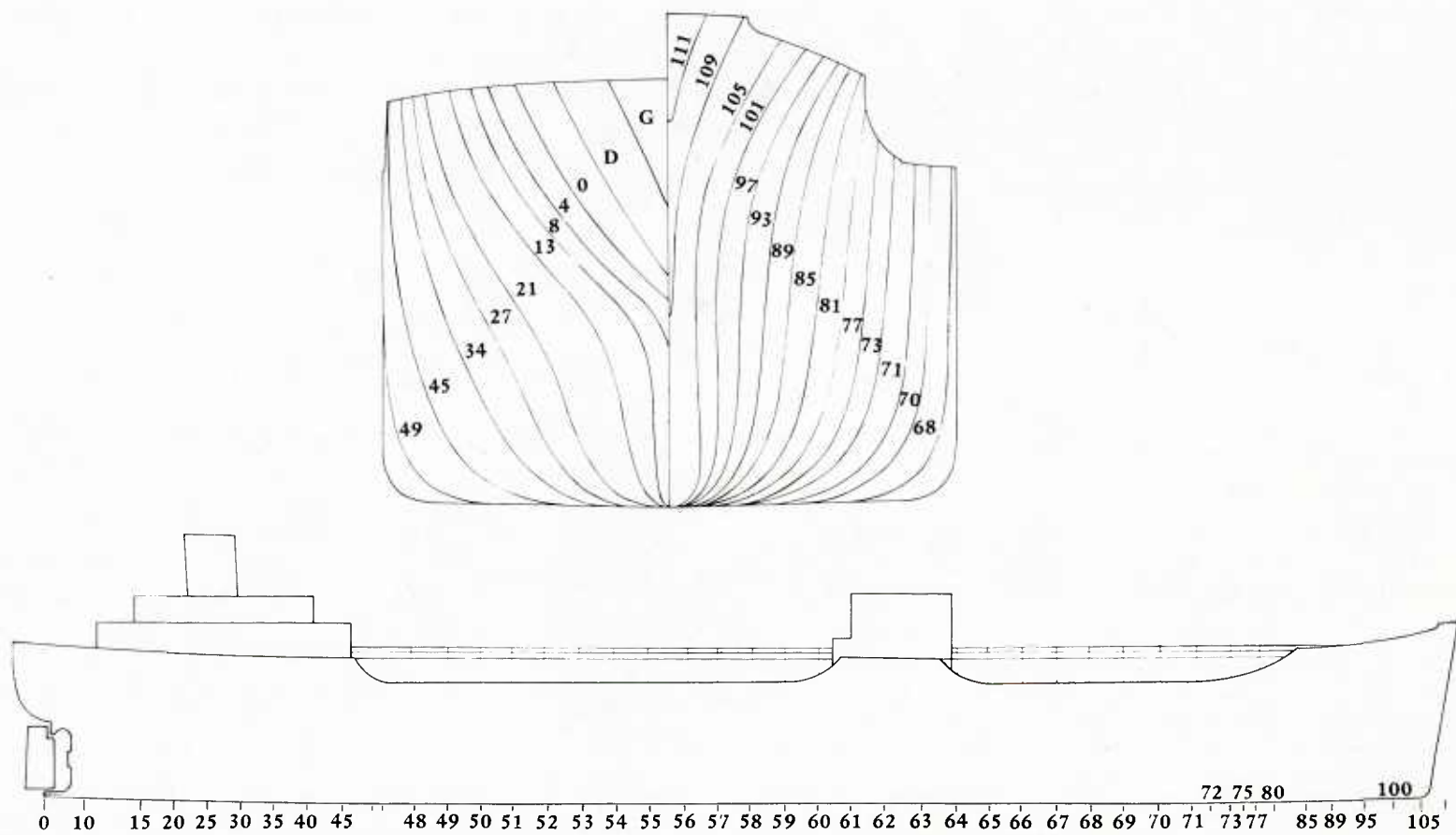
Figure 1. T-2 hull.
