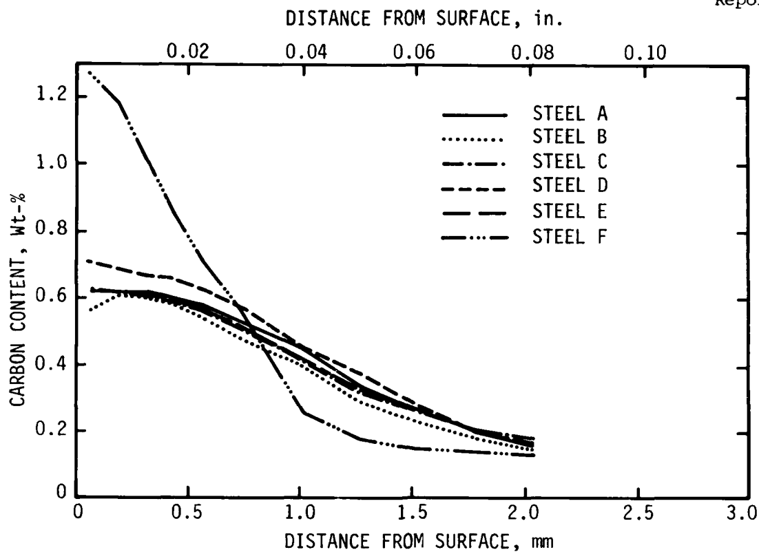
(a) Steels A - E Carburized 8.5 Hours; Steel F Carburized 7 Hours
