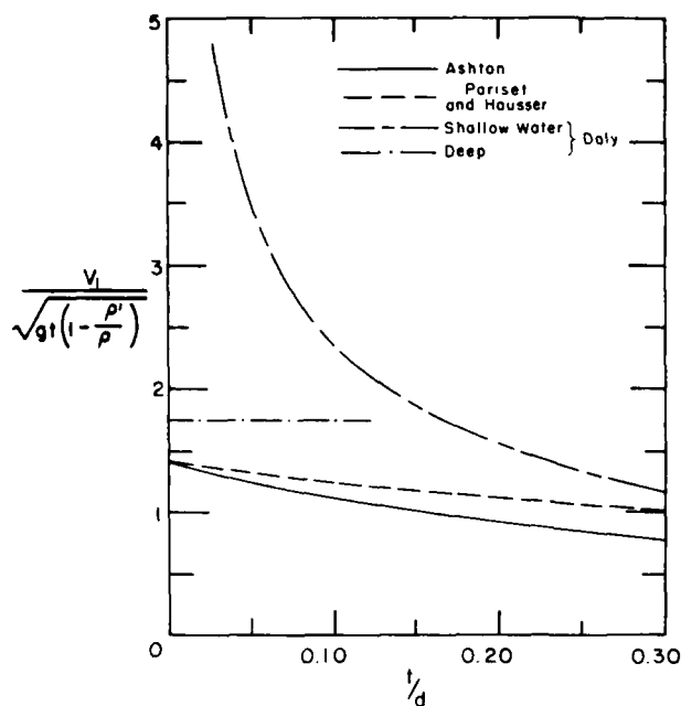
Figure 5. Four theoretical instability curves.
