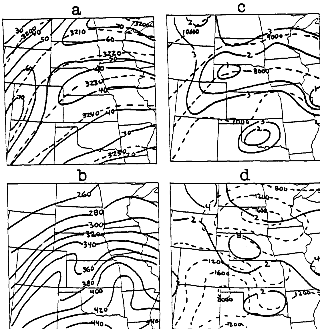
Fig. 7. Manual Analyses for 325K and 325-320K Richardson Number ( R_i ) 0000 GMT 19 March 1982 (a) Isotachs in m/s (solid) and Montgomery Stream Function in m^2/s^2 (dashed) (b) Pressure in mb. (c) Layer R_i (solid) and Mean Layer Height in m (dashed). (d) Layer Wind Shear in m/s (solid) and Layer Thickness in m (dashed).
