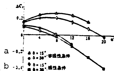
Figure 3. Quantitative lift for two-dimensional wing ground effect. a--non-linear conditions; b--linear conditions
