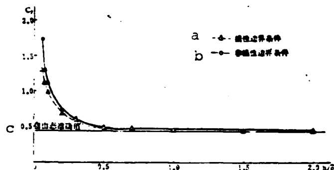
Figure 5. Two-dimensional wing ground effect lift coefficients which follow changes in ground to air distances. a--linear boundary conditions; b--non-linear boundary conditions c--free form accuracy figures
