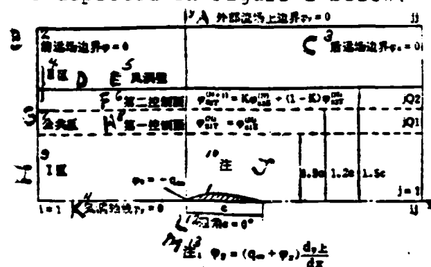
Key: A--external field of flow boundary; B--foward field of flow boundary; C--aft field of flow boundary; D--region II; E--wind tunnel; F--second control surface; G--common region; H--first control surface; I--region I; J--main; K--wind tunnel axis; L--stream angle; M--main
