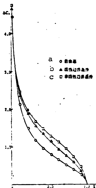
Figure 4. Two-dimensional wing with and without ground interference load distributions. a--free form; b--linear boundary conditions; c--non-linear boundary conditions
