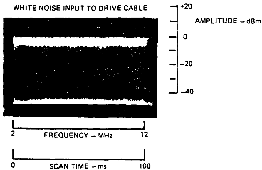
Figure 27. Inputs to Drive Cable
