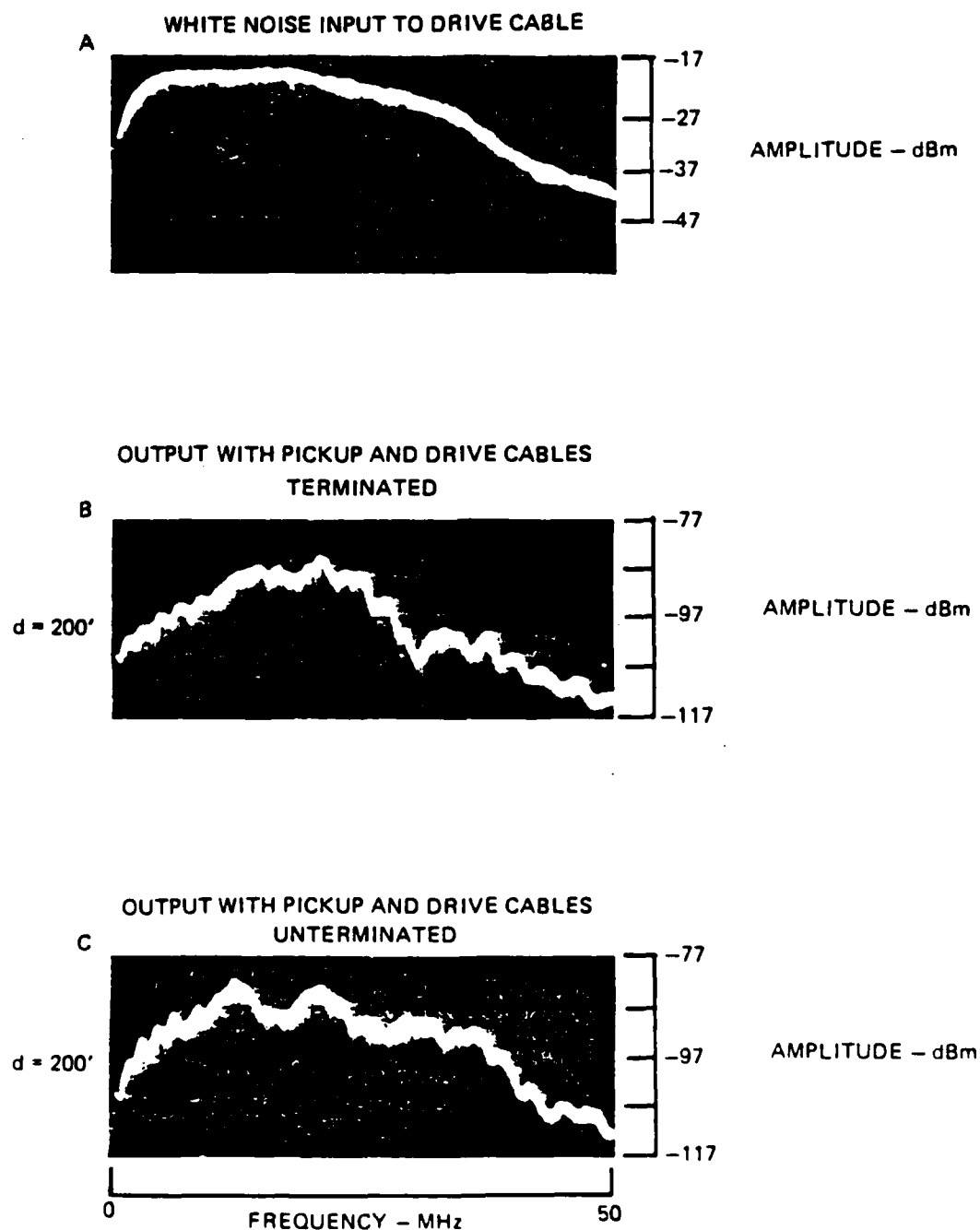
Figure 24. Coupling With Changes in Termination
