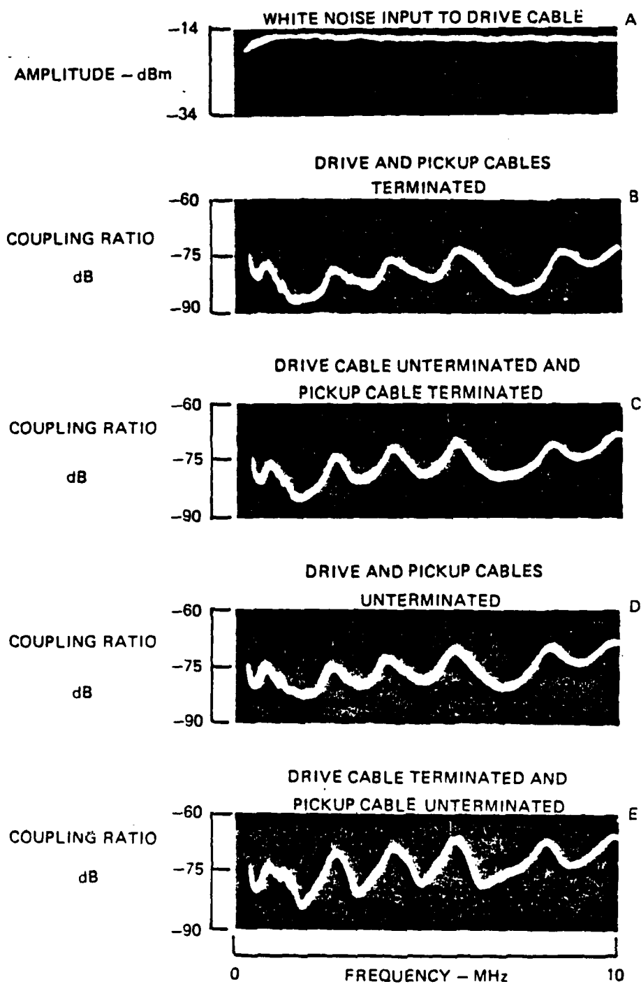
Figure 25. Coupling With Changes in Termination
