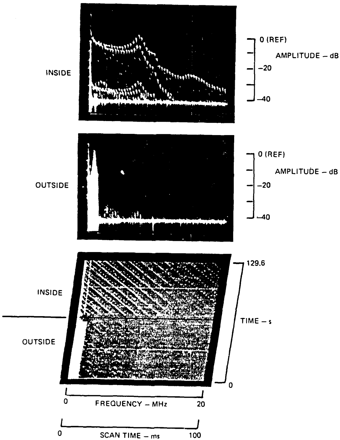
Figure 21c. Inside and Outside Currents for Configuration C
