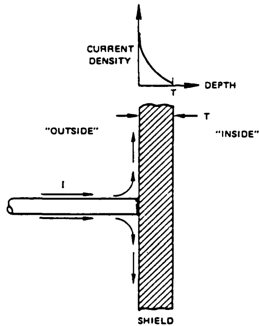
CONFINEMENT OF CONDUCTOR CURRENT TO "OUTSIDE" SURFACE BY SKIN EFFECT
