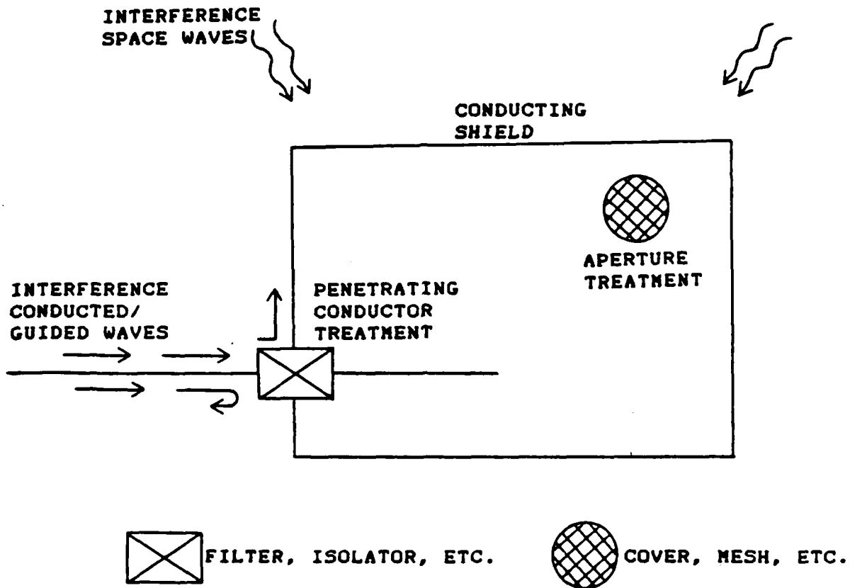
Figure 1. Generic Topological Barrier
