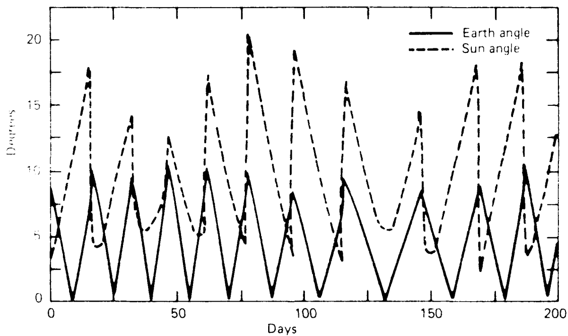
Fig. 4.4. Sun and Earth angles for A_Y = 300,000 km orbit, no lower limit on Sun angle, Earth angle < 10^\circ . Min/avg/max drift arcs = 14/18/30 days.
