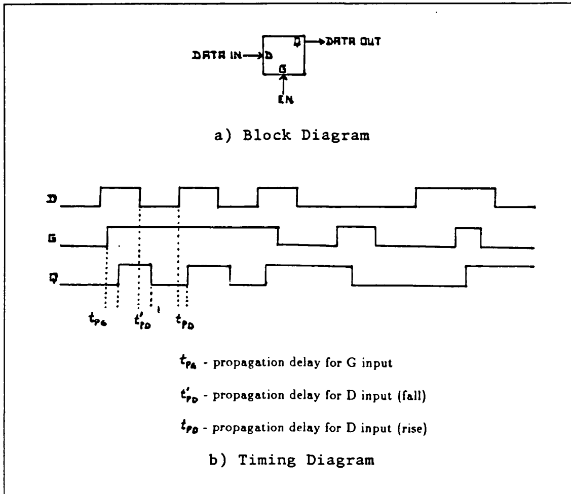
Figure 2.8 The Data Latch.
