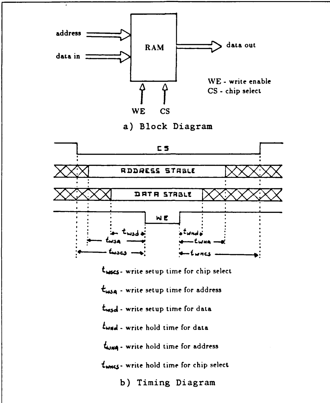
Figure 2.11 The Read-and-Write Memory.
