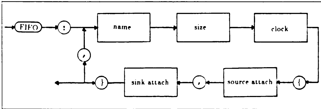
Figure 3.8 The Syntax for the FIFO Memory.
