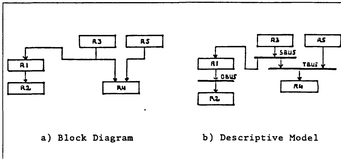
Figure 5.1 Direct Interconnection between Registers.
