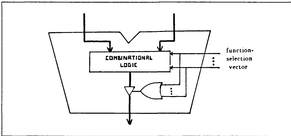
Figure 5.3 Output Gating for a Functional Unit.
