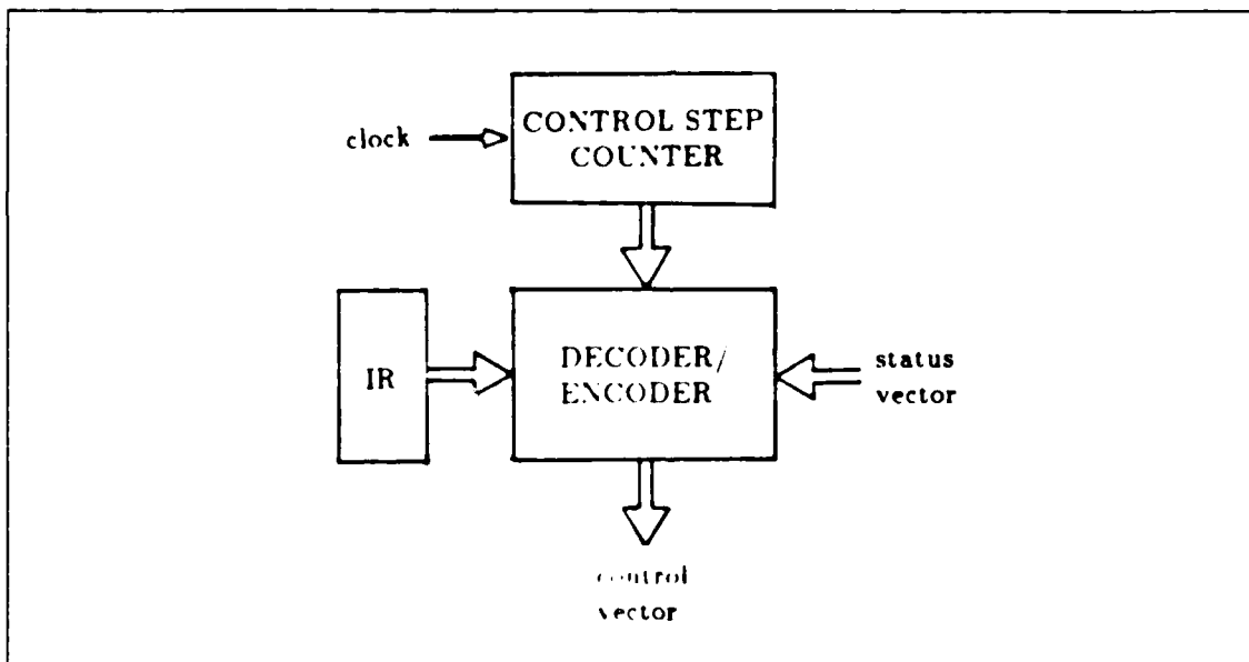
Figure 2.13 A Hardwired Control Unit Block Diagram.
