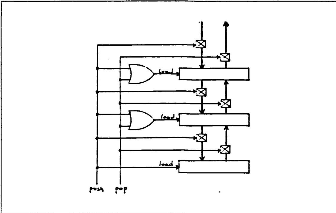
Figure 3.5 The LIFO Memory.
