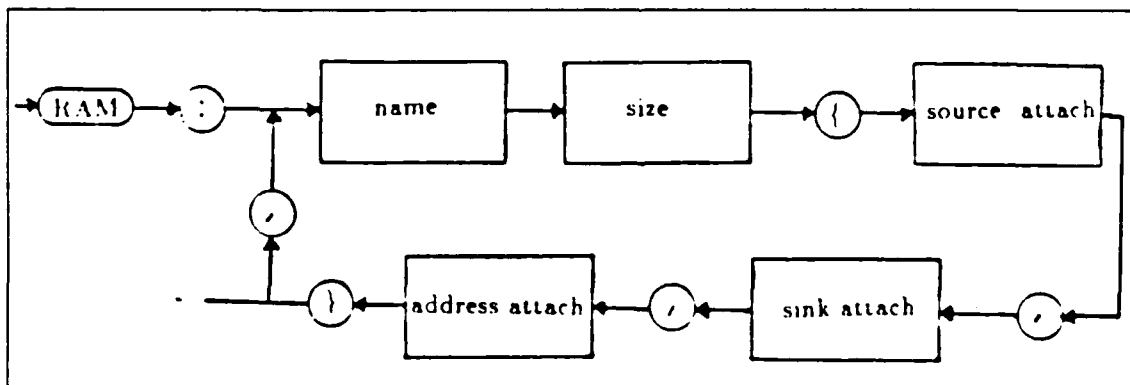
Figure 3.9 The Syntax for the Read-and-write Memory.
