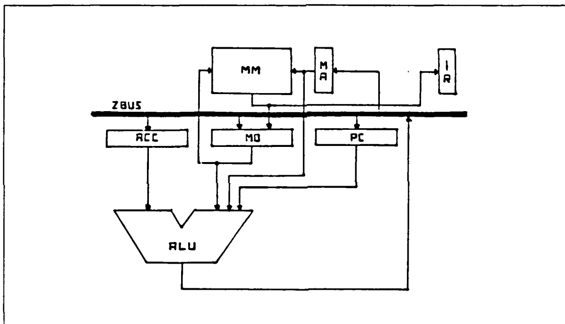
Figure 4.1 The SMI Data Flow.
