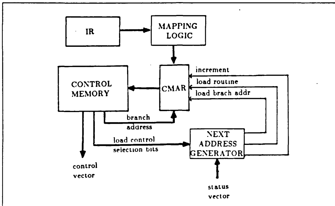
Figure 2.14 A Microprogrammed Control Unit Block Diagram.
