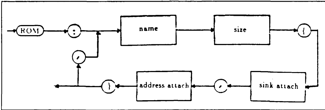
Figure 3.10 The Syntax for the Read-only Memory.
