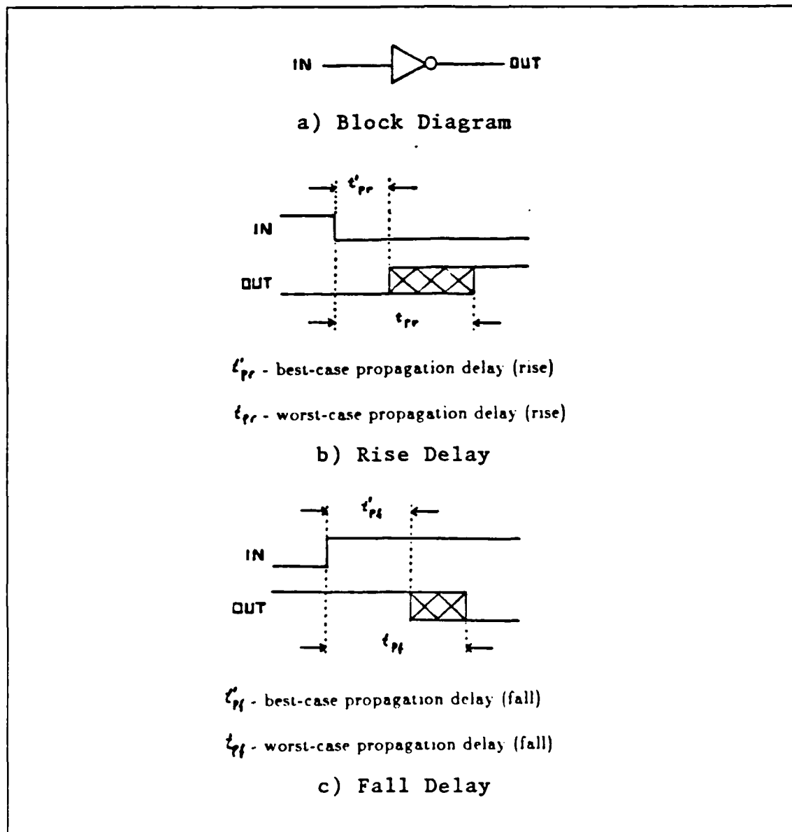
Figure 2.6 Timing Diagrams for a Simple Inverter.
