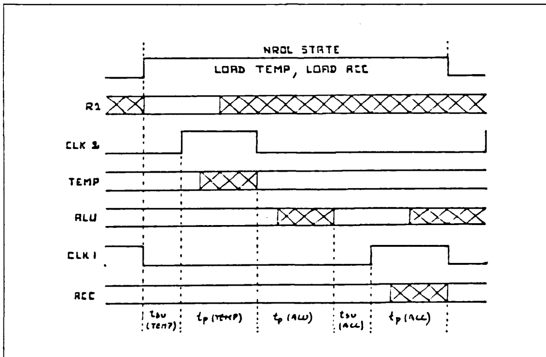
Figure 2.18 Two-phase Clock Timing Diagram.
