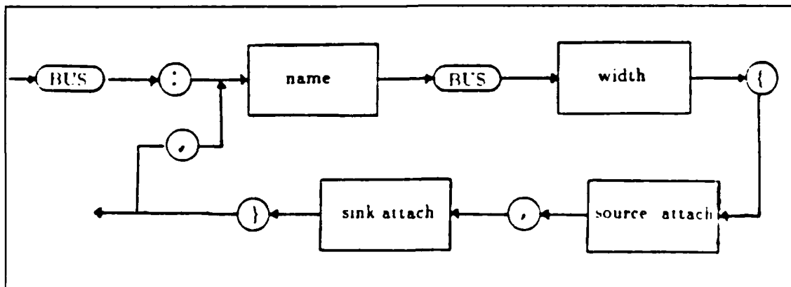
Figure 3.3 The Syntax for Bus.
