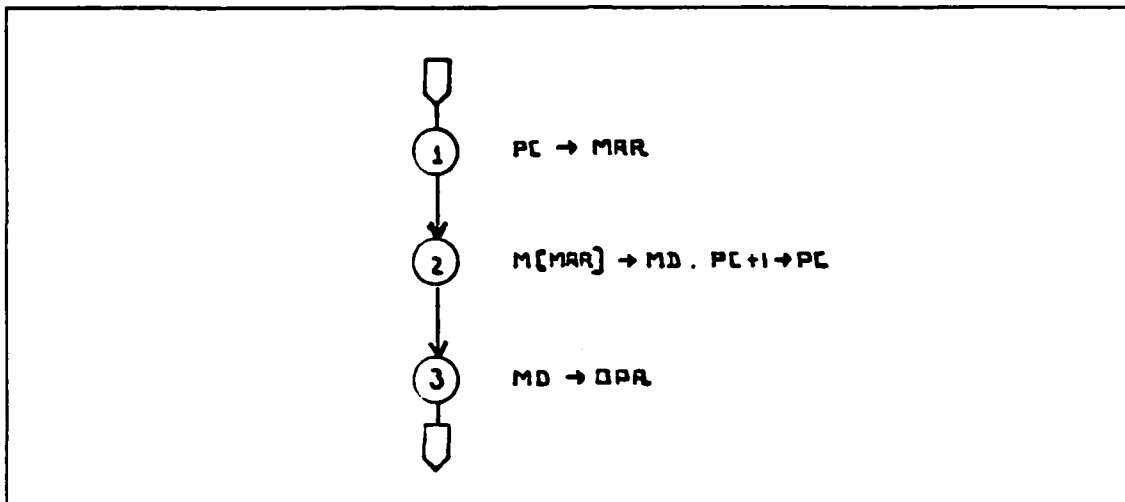
Figure 4.2 Example of a Fetch Cycle State Diagram.
