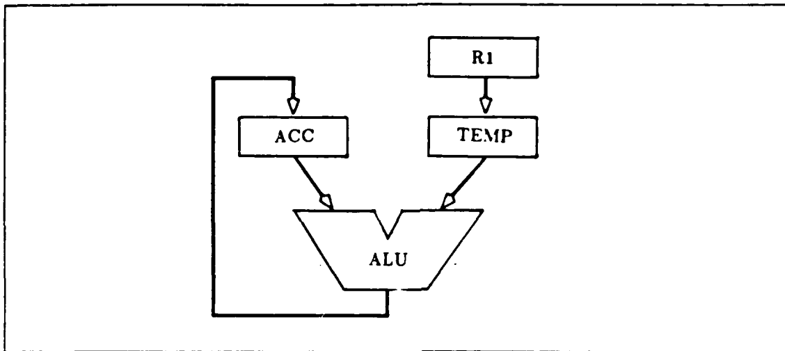
Figure 2.15 Part of a Data Flow.
