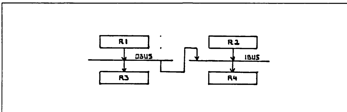
Figure 5.6 EXAMP Data Flow.
