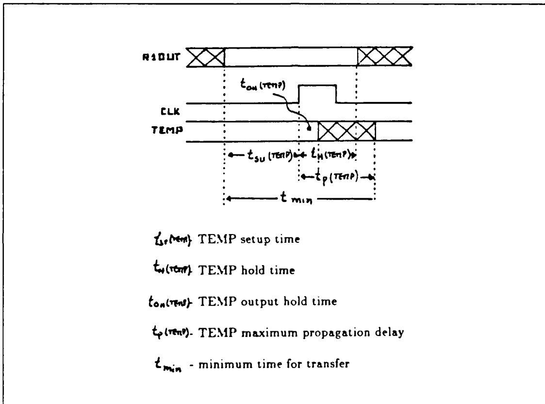
Figure 2.16 Timing Diagram for a Simple Transfer.
