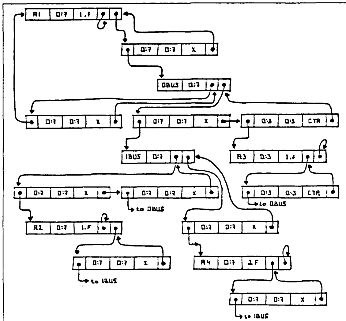
Figure 5.7 Storage of Examp.
