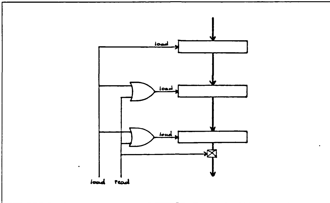
Figure 3.7 The FIFO Memory.
