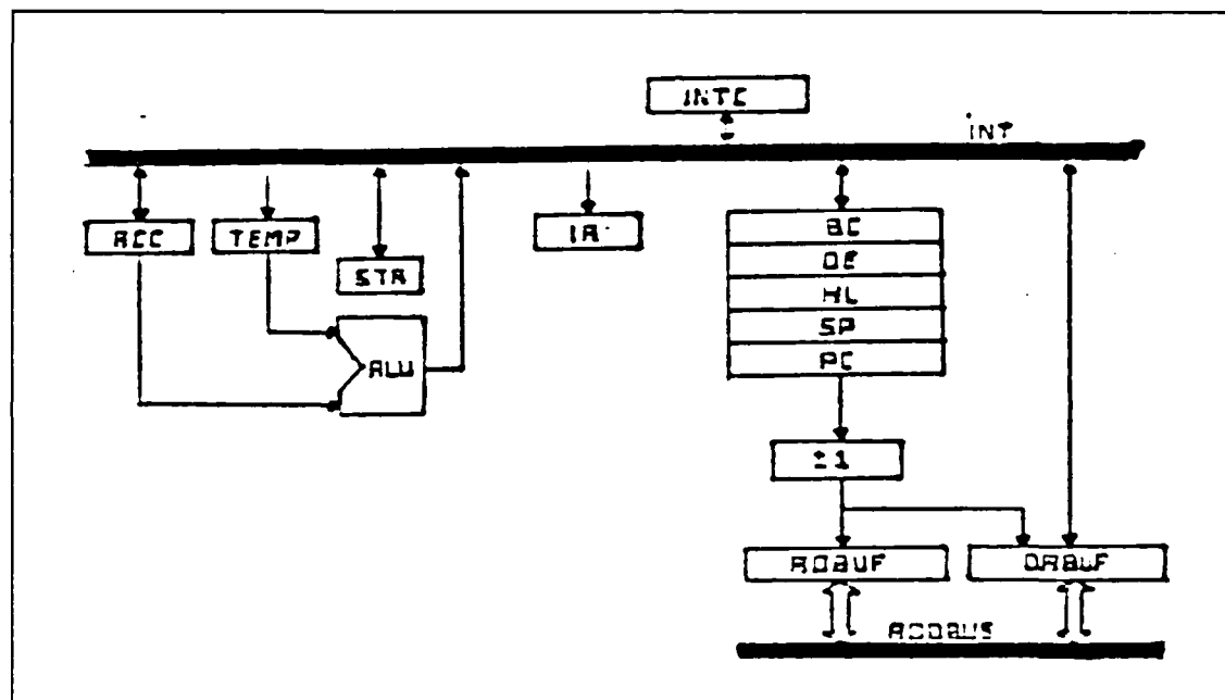
Figure 4.5 The 8085A Data Flow Diagram.
