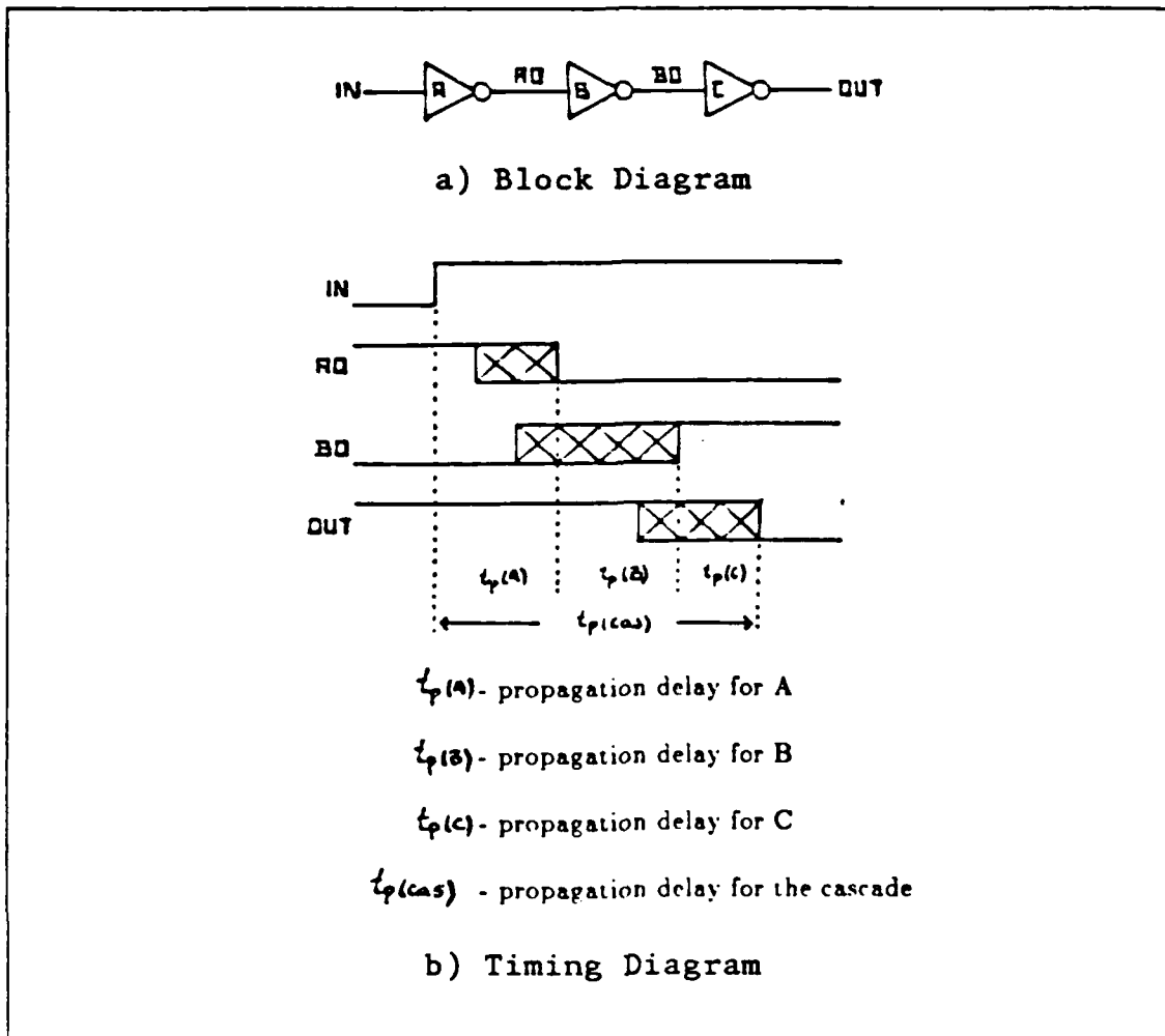
Figure 2.7 A Cascade of Inverters.
