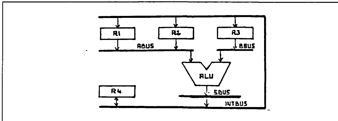
Figure 5.4 Data Paths Including Functional Units.
