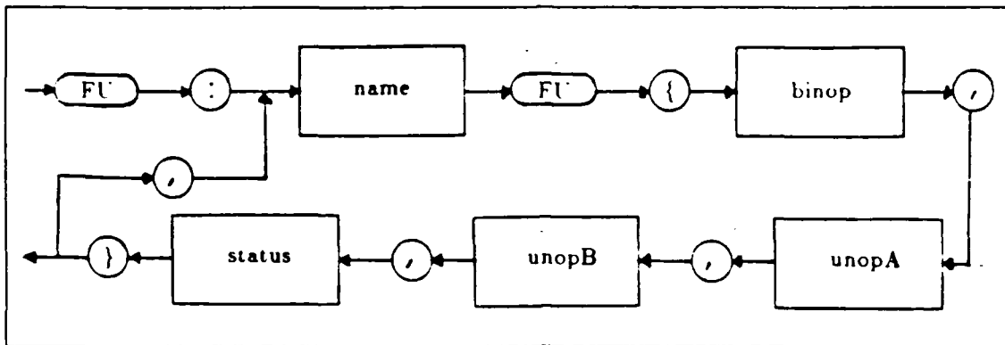
Figure 3.11 The Syntax for the Functional Unit.
