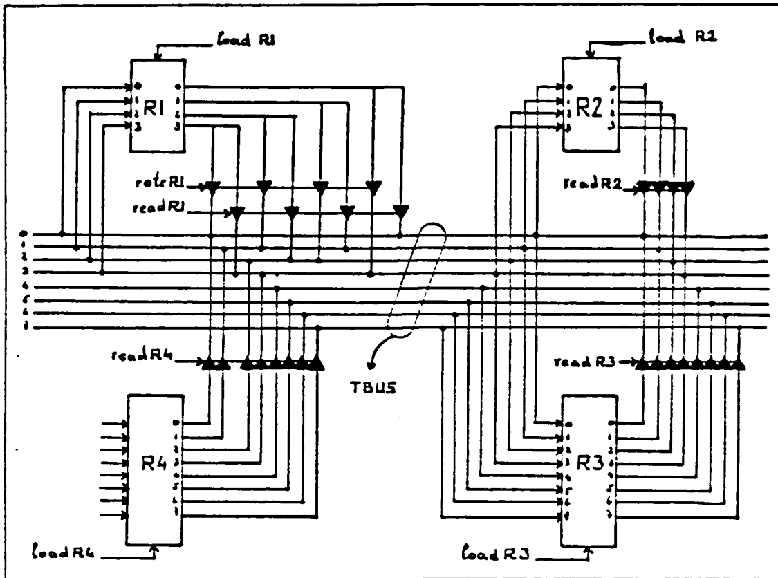
Figure 3.1 Example of Bus Attachments.
