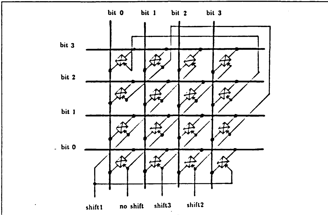
Figure 3.2 The Barrel Shifter.
