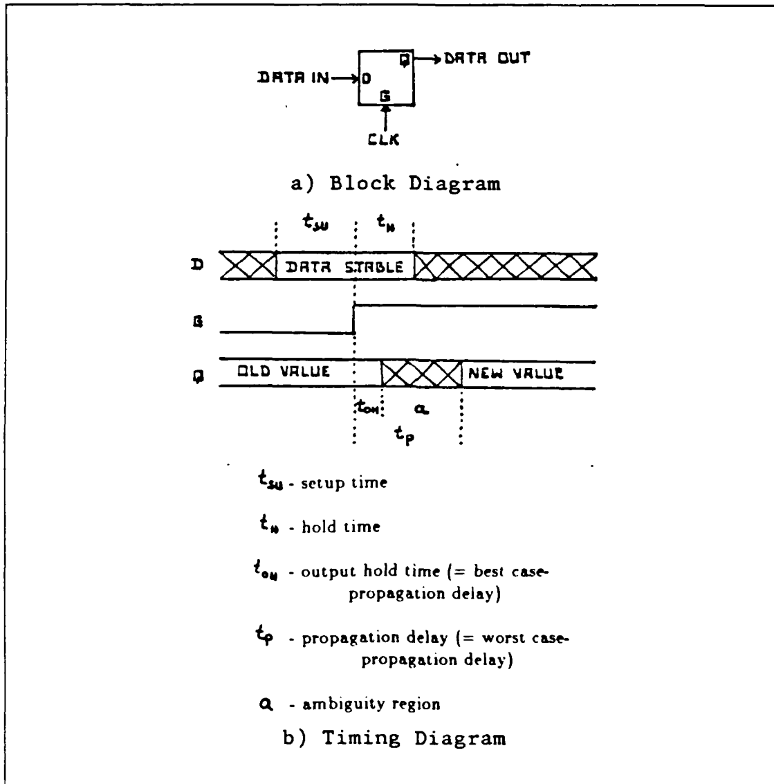
Figure 2.9 The Edge-Triggered Flip-Flop.
