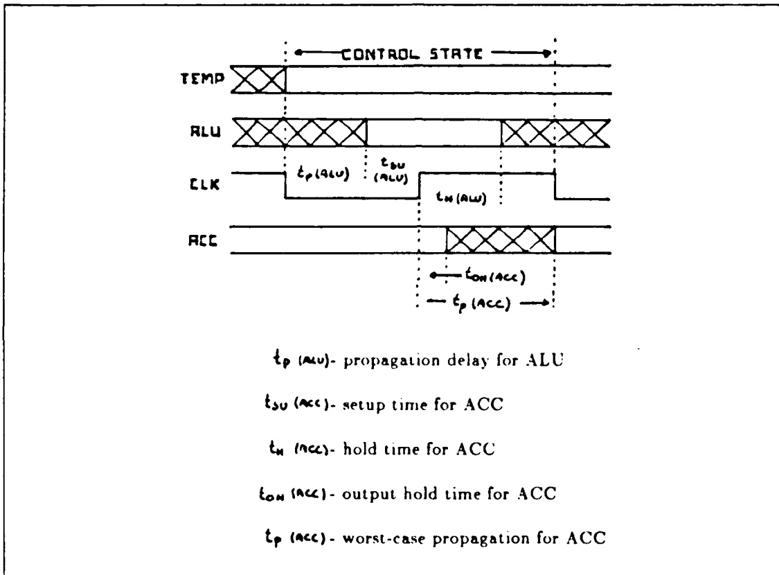
Figure 2.17 Timing Diagram for a Functional Transfer.
