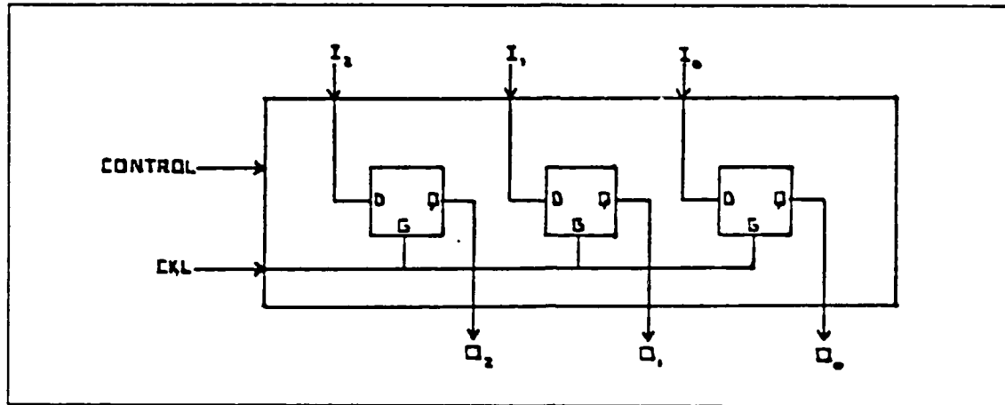
Figure 2.10 A Register as an Array of Flip-Flops.
