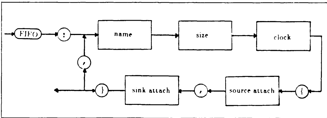
fifo
