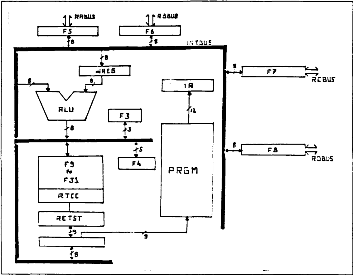
Figure 4.4 The PIC 1650 Data Flow.
