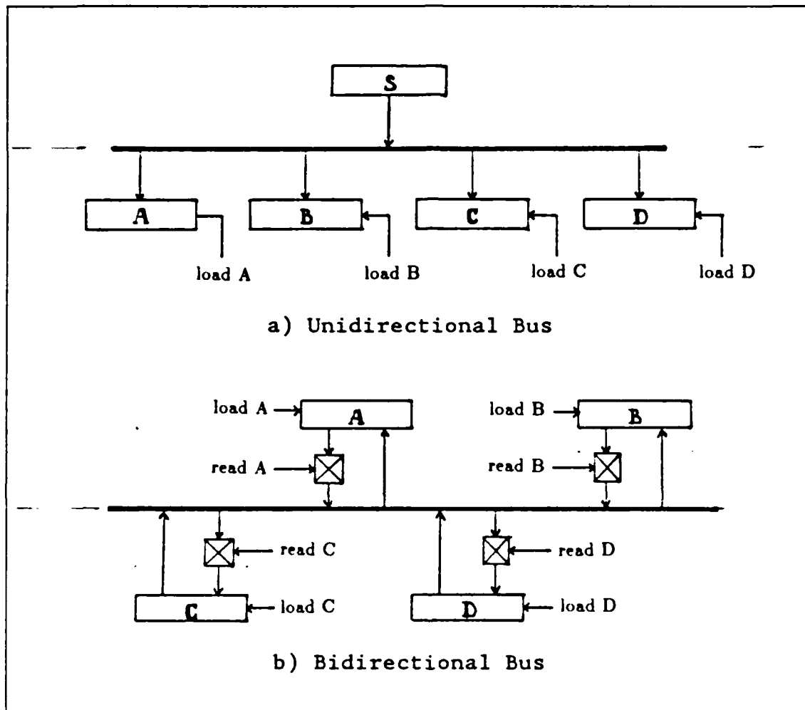
Figure 2.3 A Bus System.
