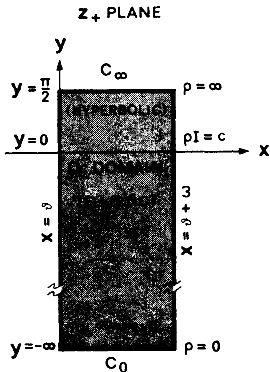
Figure 3-3. Mapping of the wave domain, \Omega into the z_+ plane by the characteristic transformation.
