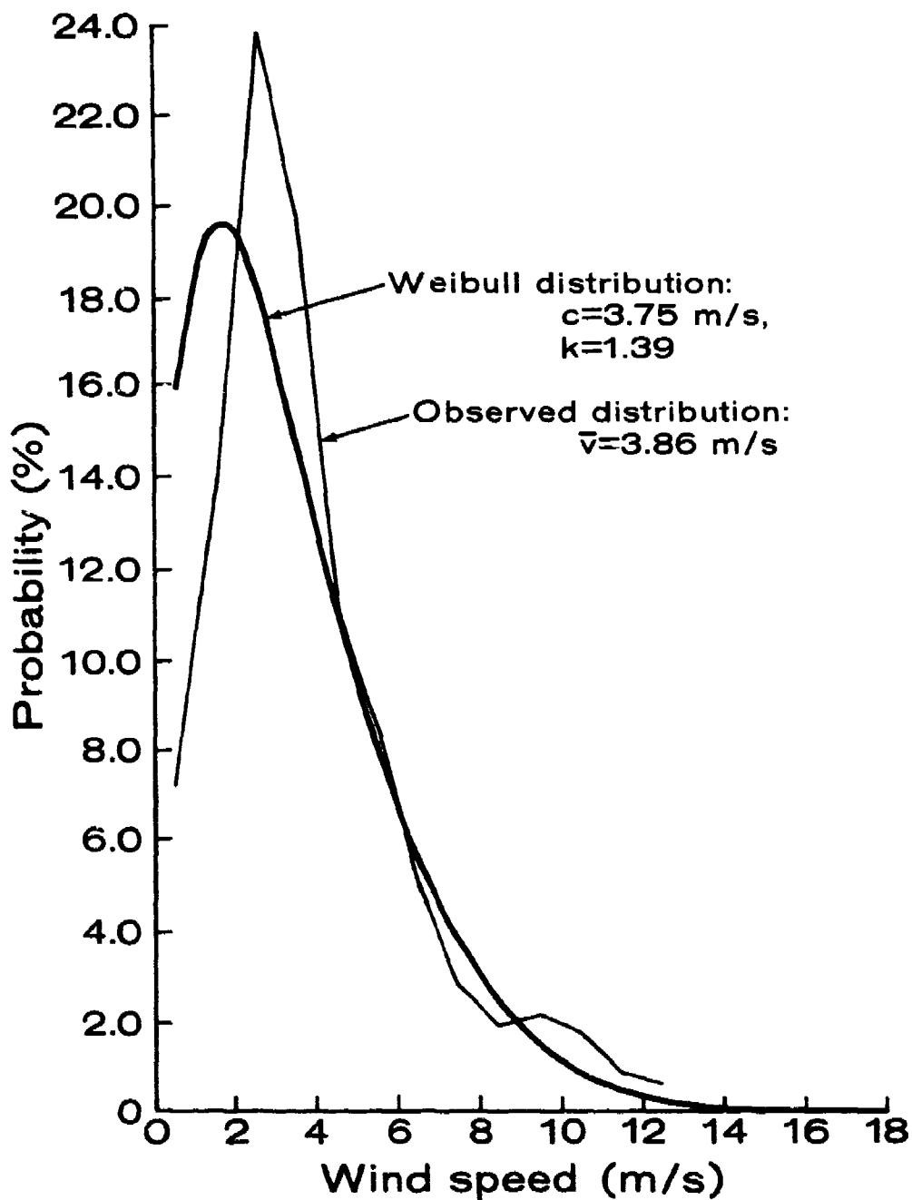
Fig. 12. Probability distribution and corresponding Weibull curve for data from 300 ft level of Tower 300. Number of observations: 2826.
