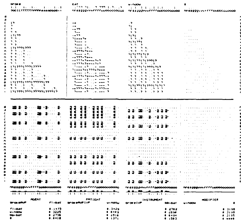
Figure 13. State of the model after processing the sentence The bat broke the window . For this sentence, the black background on the Agent units shows which units would be active in the pattern for flying bat as Agent of the agentive (AVP) reading of broke . The black background on the Instrument units indicates the units that would be active in the pattern for baseball bat as Instrument of the instrumental (IVP) reading of broke . The black background on the Patient units indicates the units that would be active in either the pattern appropriate for window as Patient of the agentive reading of broke or in the instrumental reading of broke .
