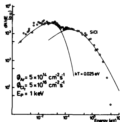
Figure 2. Total fit of the kinetic energy distribution of SiCl (m/e=63) particles for the parameters as given in the figure. At low energy a Maxwell-Boltzmann distribution at 300 K is indicated, while at higher energies, above 0.1 eV, a collision cascade distribution is given with an U_0 = 0.3 \text{ eV} .
