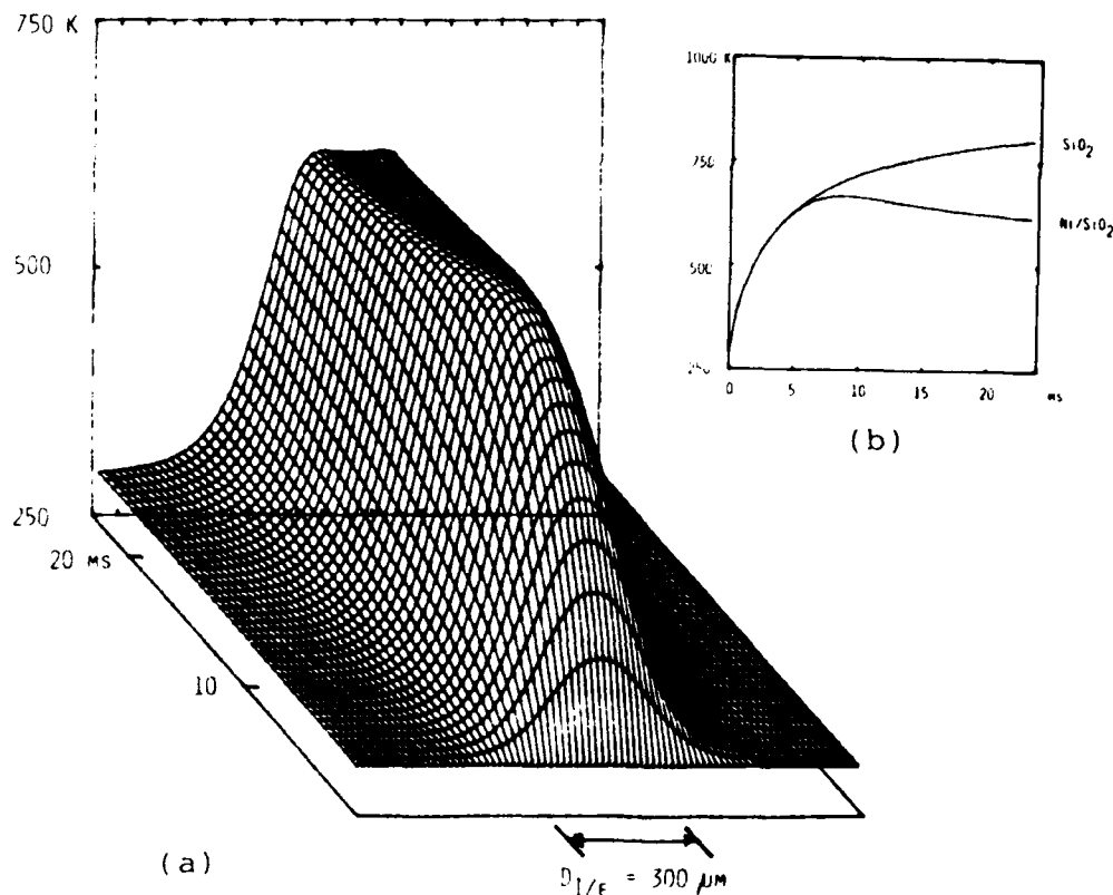
Fig. 1. Temperature of \text{Ni/SiO}_2 surface for an incident laser power, P = 1 \text{ W} ; D_{1/e} = 300 \mu\text{m} . a) Surface temperature distribution as a function of irradiation time with Ni deposition. b) Axial surface temperature with ( \text{Ni/SiO}_2 ) and without ( \text{SiO}_2 ) deposition.
