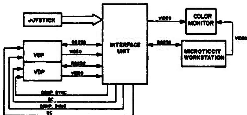
Figure 2-1. FULL CONFIGURATION
