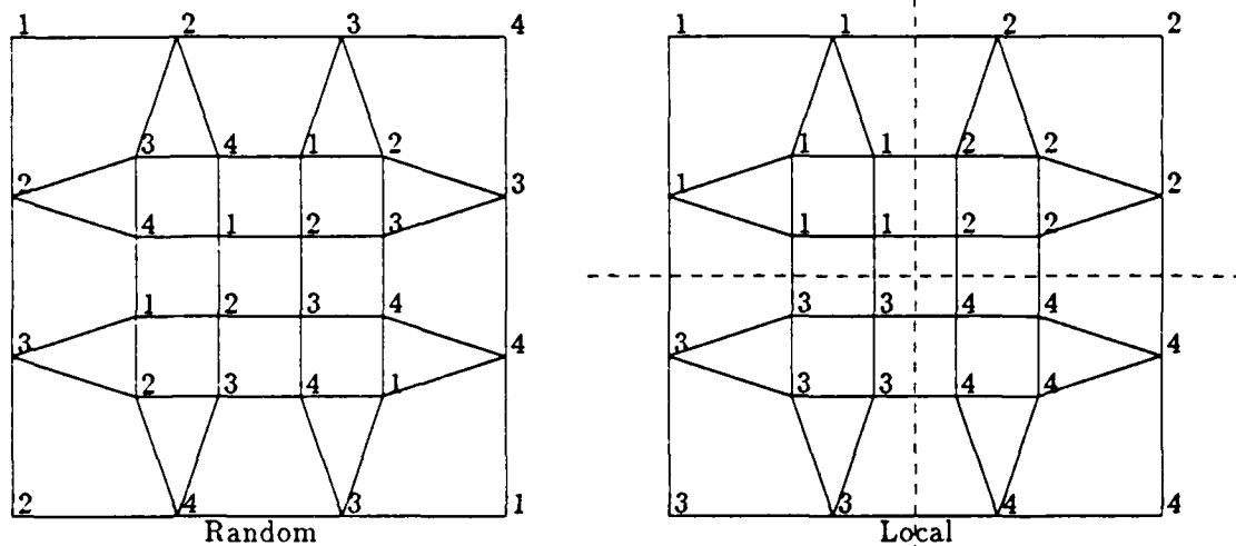
Figure 3: Random and local mapping of vertices onto processors. Mappings for a 4 processor system are shown; dashes in the local mapping show the "clumps".
