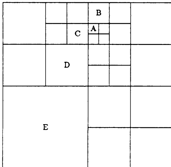
Figure 2: To refine mesh cell "A", cells "B" and "C" must first be refined. To refine cell "C", cell "D" must be refined. Similarly for "E".
