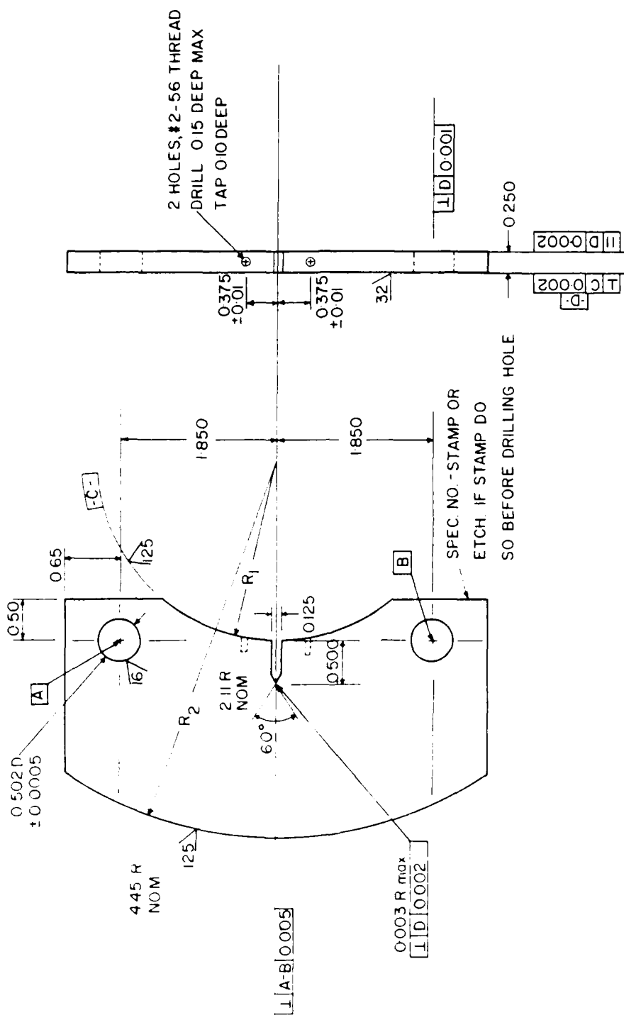
Figure 2: Fatigue crack growth specimen dimensions.
