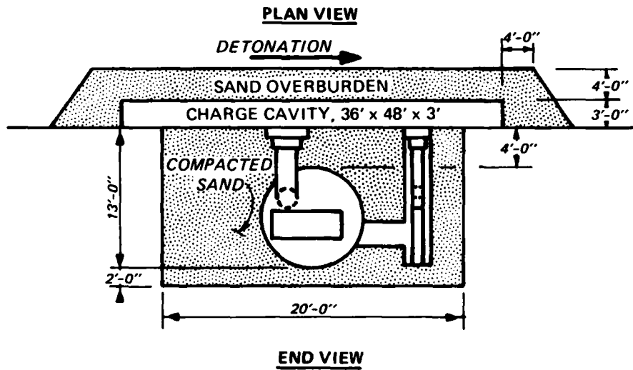
Figure 2.4. Test configuration.
