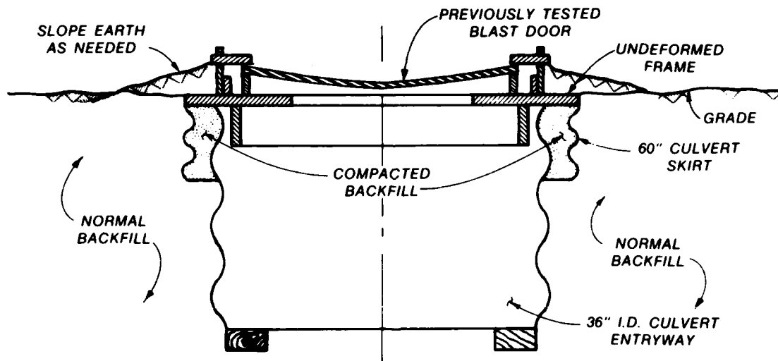
ELEVATION VIEW
