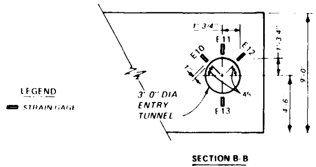
Figure 2.10. Instrumentation locations.
