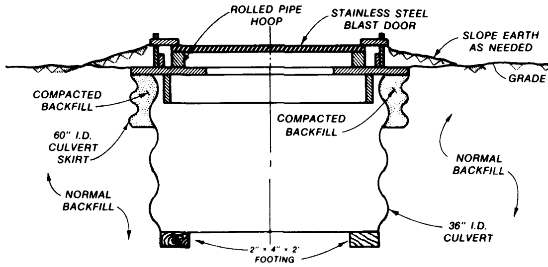
ELEVATION VIEW
