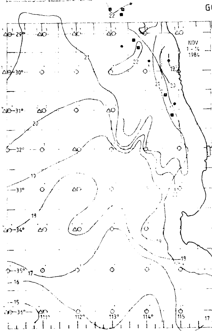
Fig 5(a). SST Analysis for Nov.1-14 1984.
