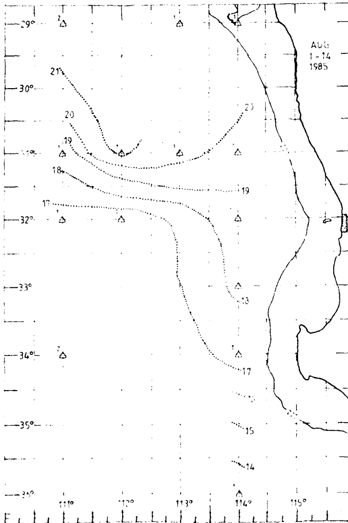
Fig 14(a). SST Analysis for Aug.1-14 1985.
