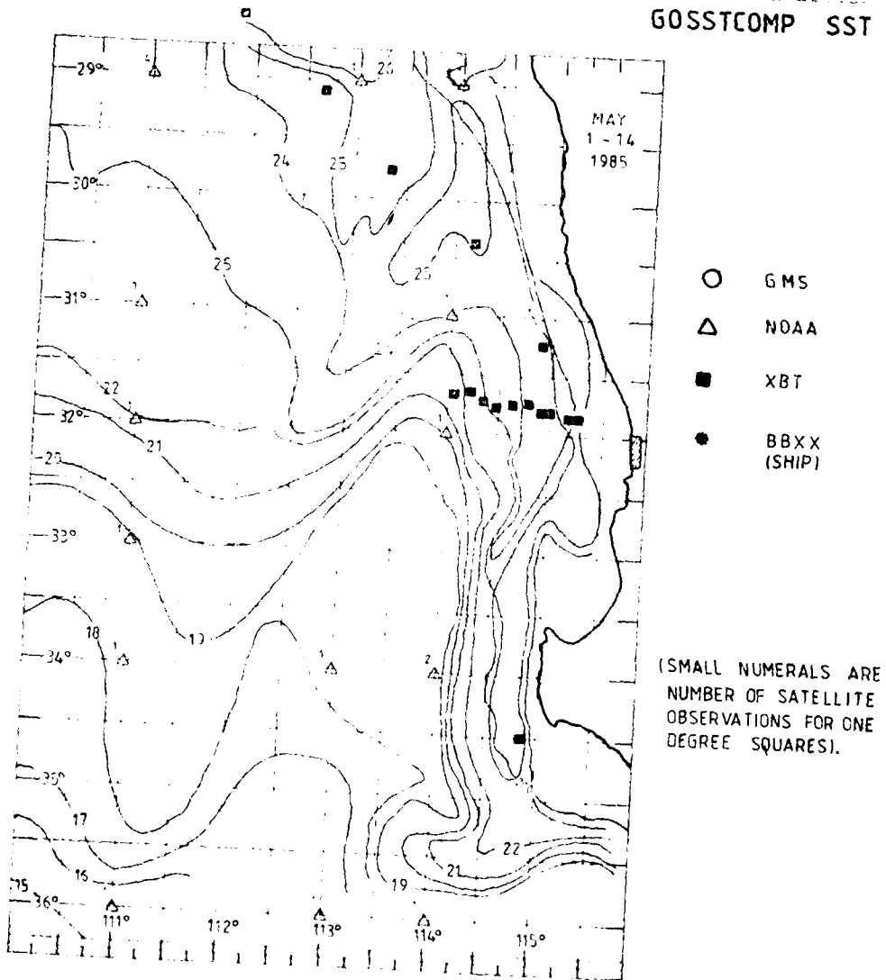
Fig.11(a). SST Analysis for May 1-14 1985.
