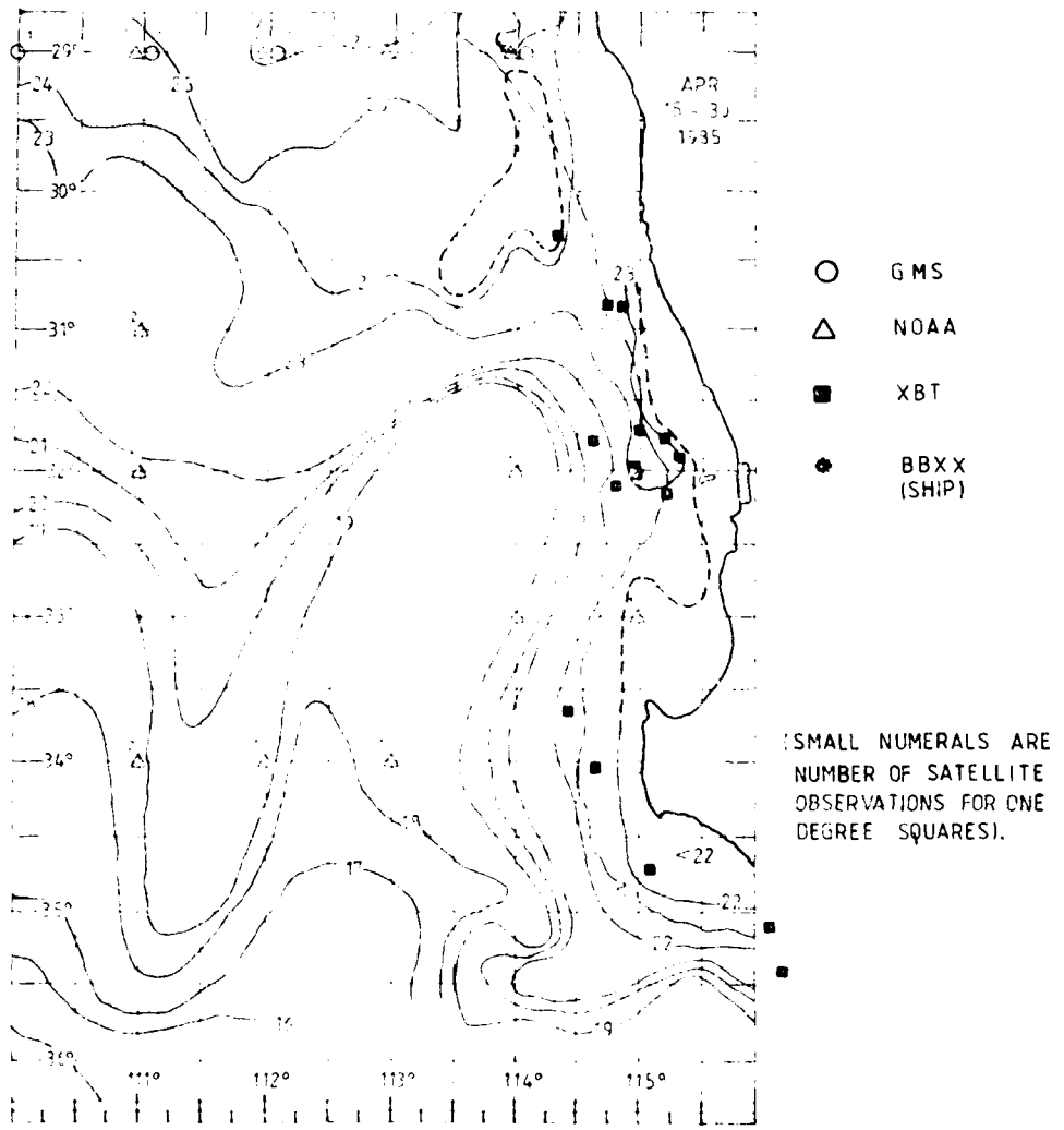
Fig 10(b). SST Analysis for Apr. 15-30 1985.
