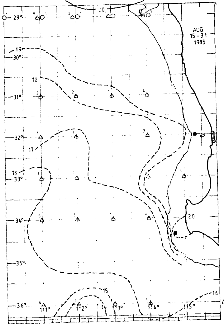
Fig.14(b). SST Analysis for Aug.15-31 1985.
