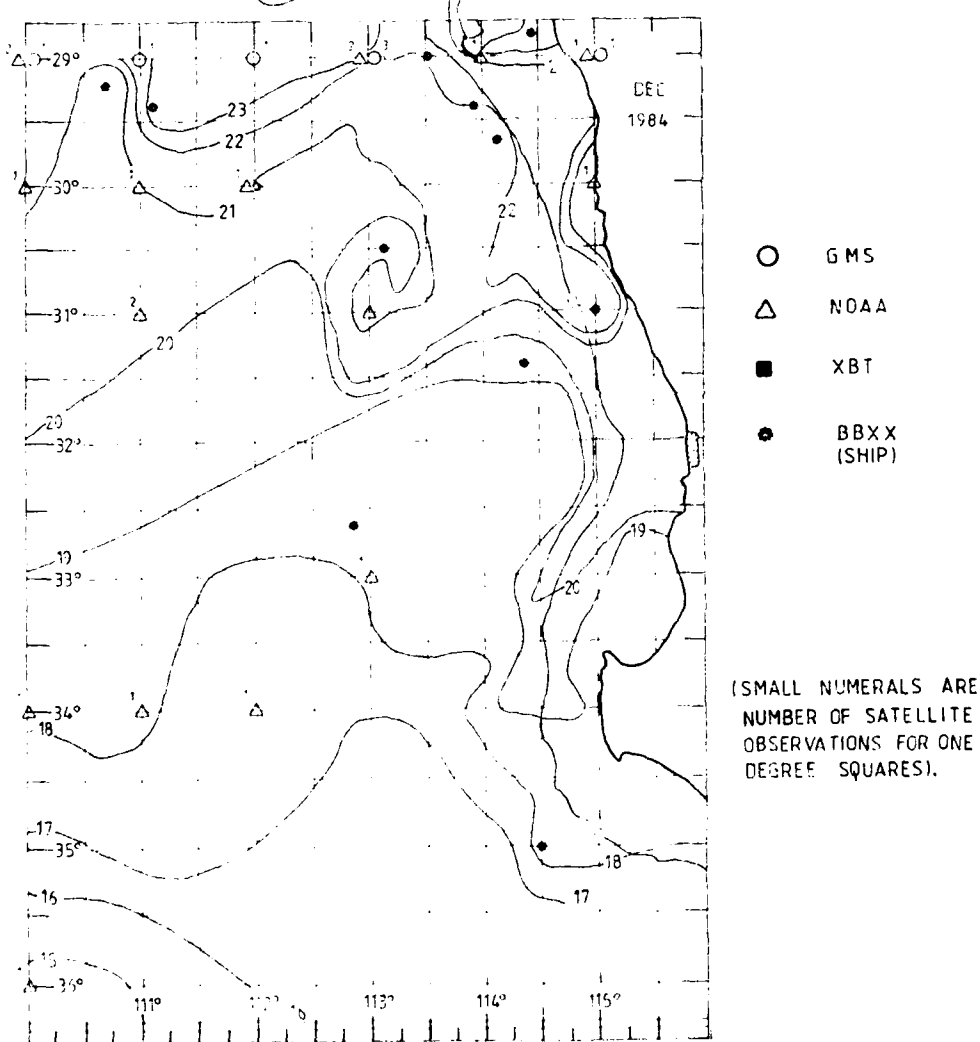
Fig. 6. SST Analysis for December 1984.
