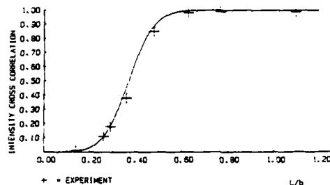
Fig. 4. Peak values of the intensity cross correlation measured at angles (-\theta_0, \theta_0) as a function of L/b ( \sin \theta_0 \approx \lambda/b ).
