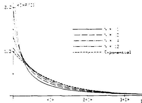
Fig. 3. Probability densities of the doubly scattered intensity from Eq. (16) for various values of the N parameter. A negative-exponential distribution is shown for comparison.
