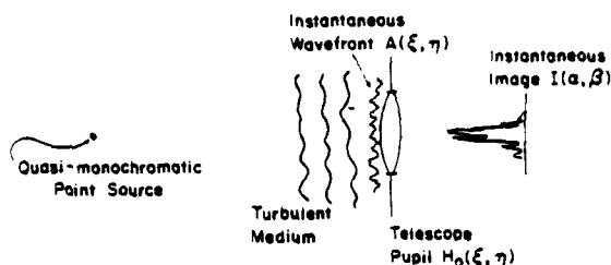
Fig. 7.3. The formation of an instantaneous image of a point source through the atmosphere
