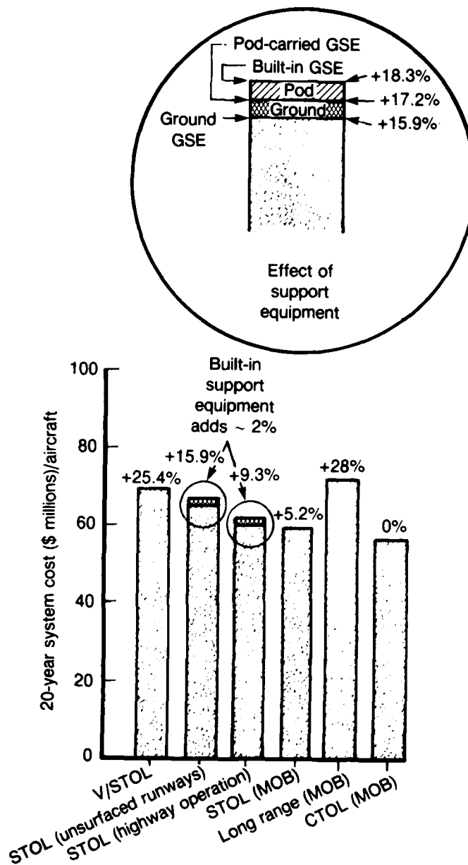
Fig. 4—Life cycle costs of aircraft designs under different basing concepts
