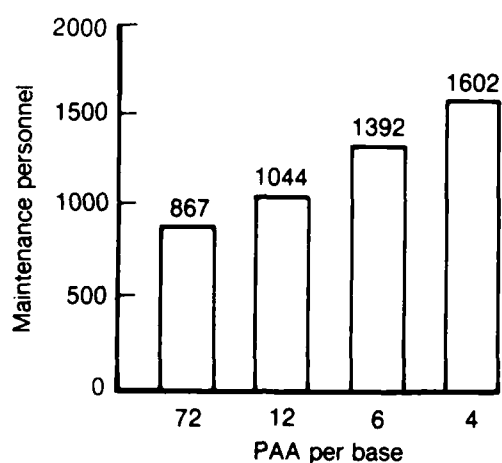
Fig. 3—Maintenance personnel needed to sustain constant sortie rate with 72 fighters
