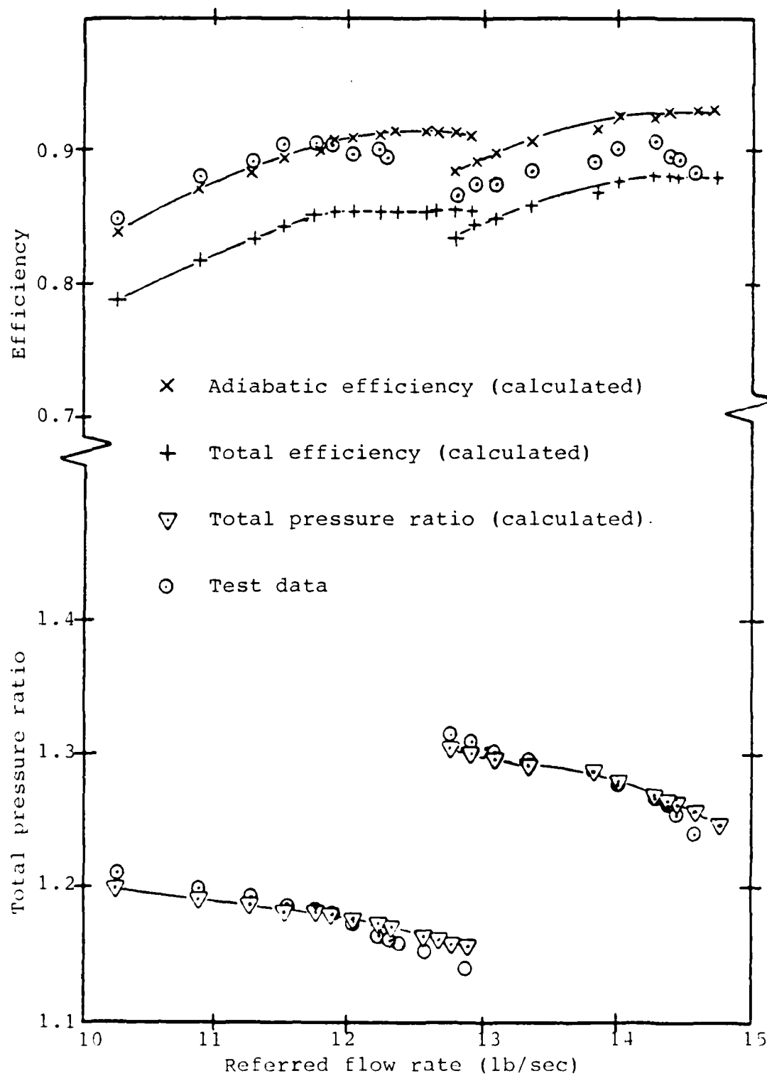
Figure 17. Calculated and measured compressor performance maps at 60% and 70% design speed.
