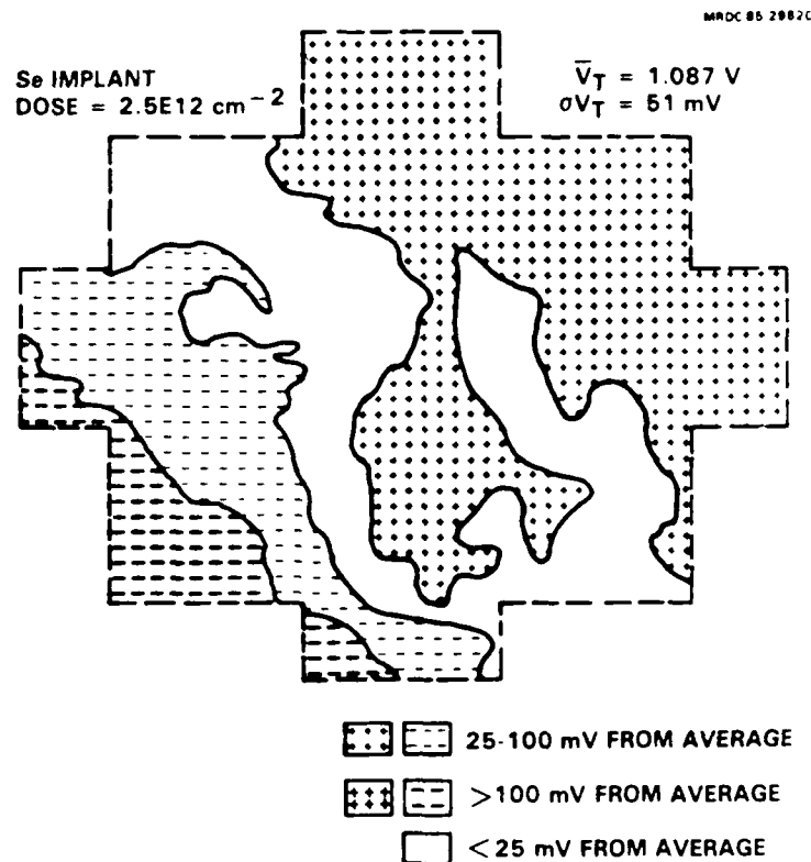
Fig. 2.3-1 Implant uniformity, Se implant.
