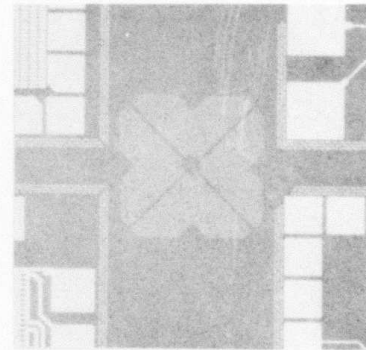
ALIGNMENT MARK
