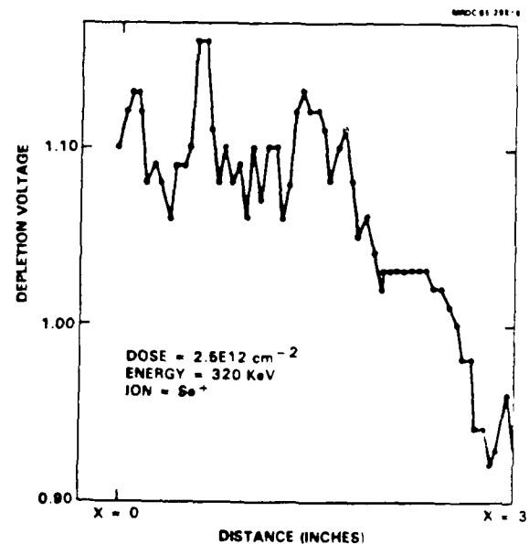
Fig. 2.3-3 Implant uniformity, Se implant.
