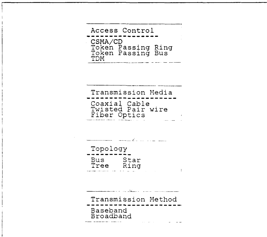
Figure 5.1 Taxonomy Tree.
