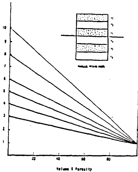
PARALLEL CAPACITIVE MIXING
