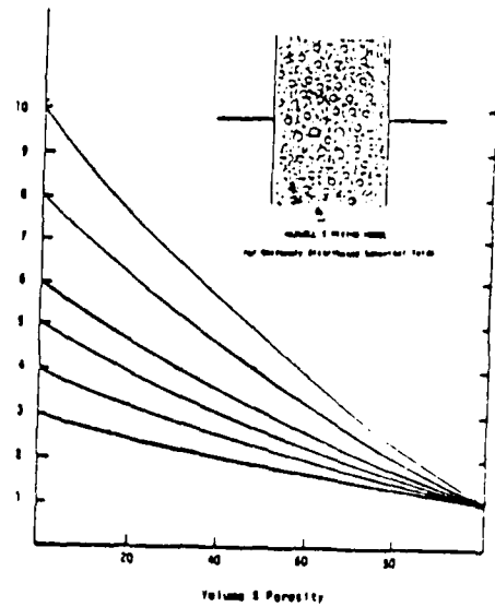
MAXWELL'S MIXING MODEL (Spherical, Homogeneously Distributed Pores in Continuous Matrix)
