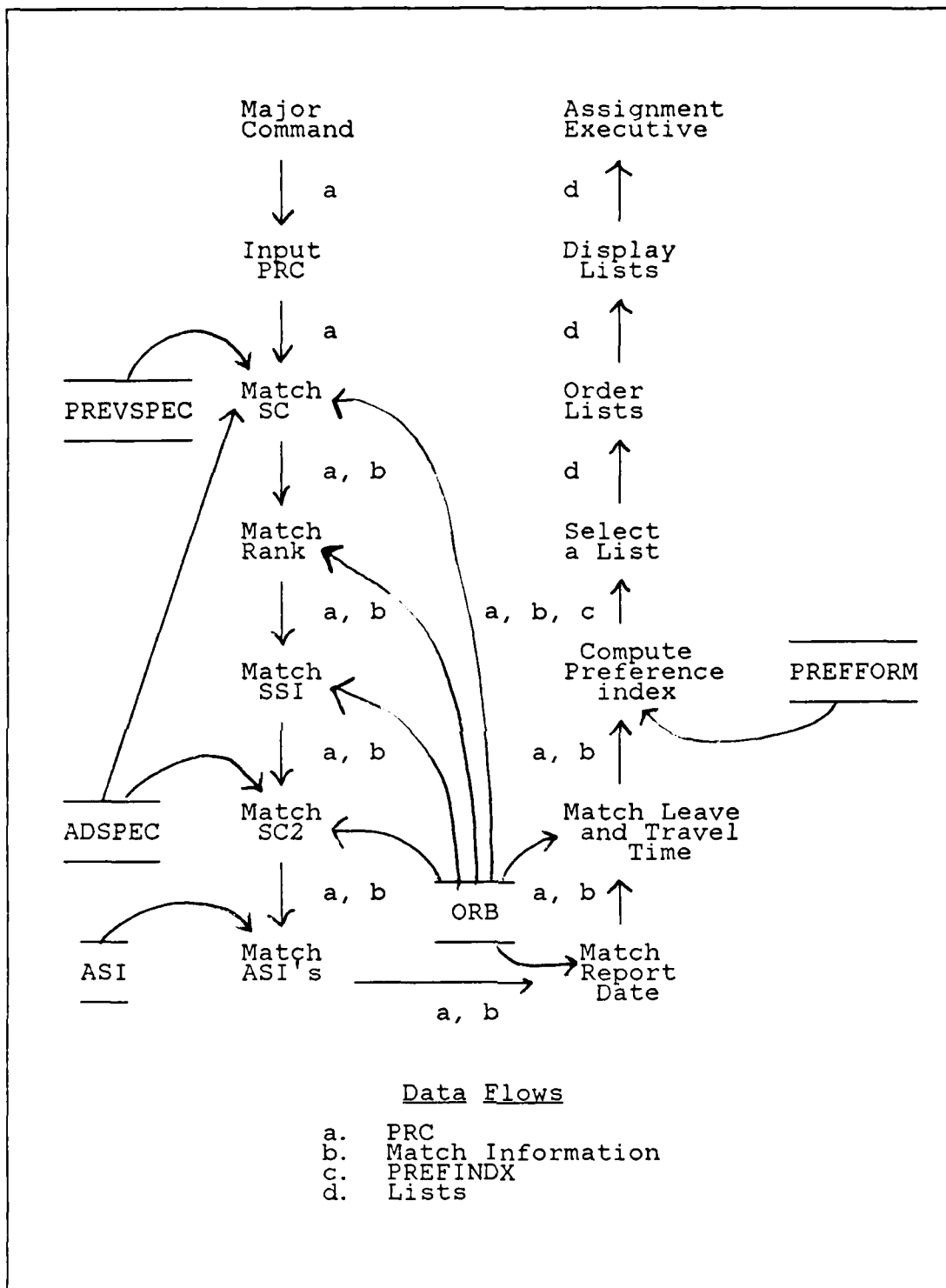
Figure 3.1 Program Flow.
