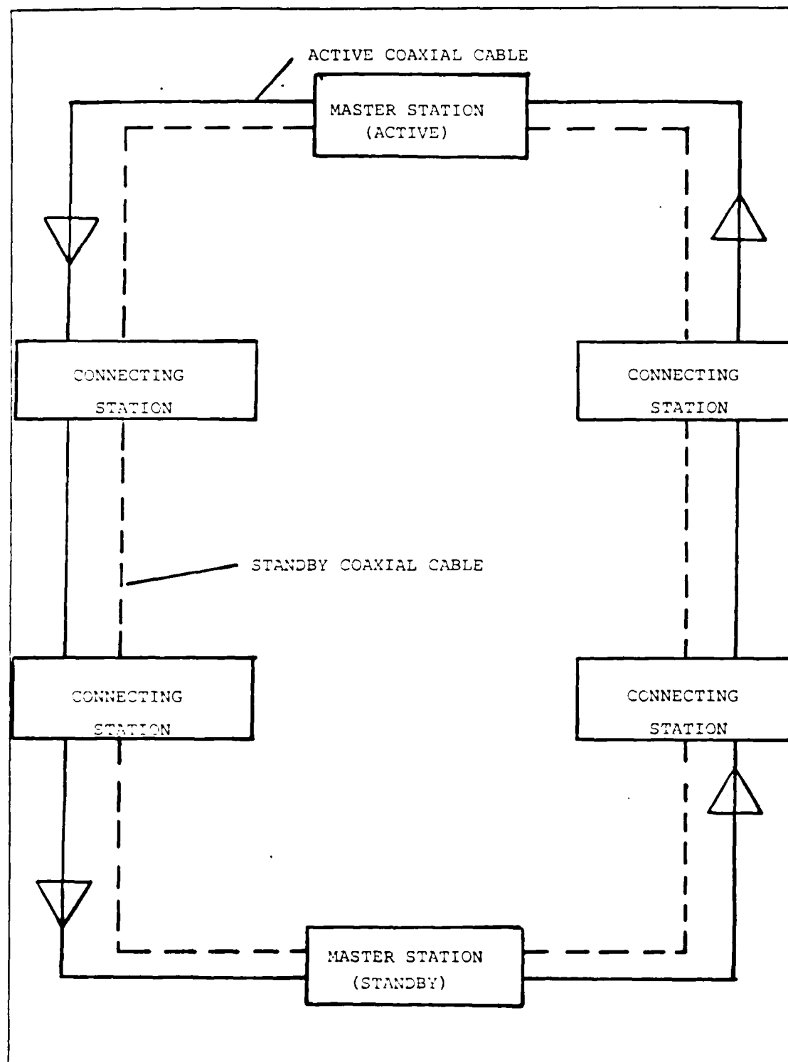
Figure 4.1 SNTI Network Architecture.
