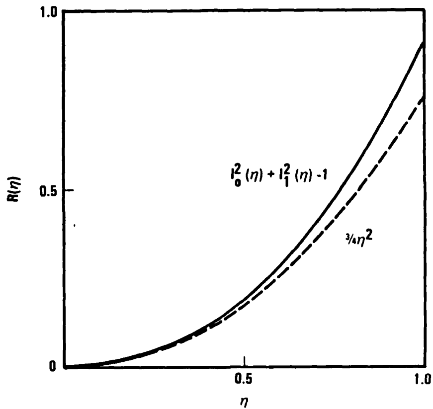
Figure 2. Reflectivity verse \eta in linear scale (Equation (17)).
