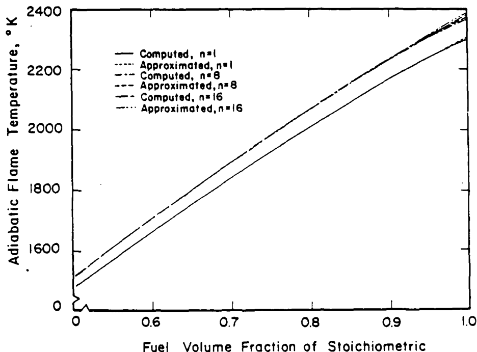
FIGURE 1. Adiabatic flame temperature of paraffin family, C_nH_{2n+1} , as function of fuel air ratio and number of carbon atoms of fuel for reaction pressure of 100 atm.
