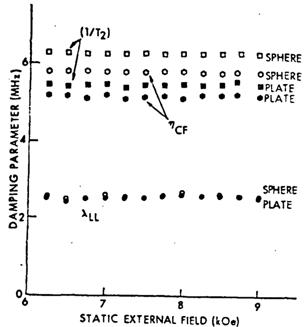
Fig. 1 Various phenomenological damping parameters as a function of applied static field for a YIG sphere and a thin plate.
