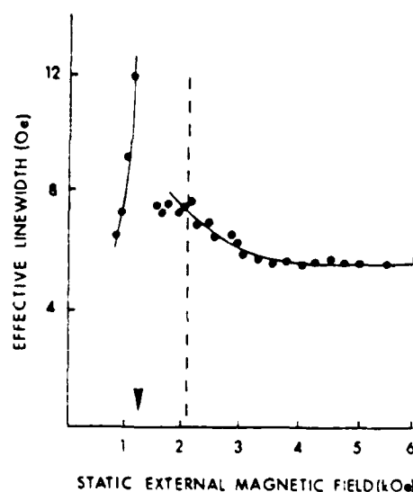
Fig. 1. Effective linewidth as a function of applied field for single crystal \text{Zn}_2\text{-Y} sphere with planar anisotropy. The pointer above the field axis represents the position of FMR field at 9.9 GHz. The broken vertical line indicates the field at which the bottom of the spin wave manifold lies at 9.9 GHz.
