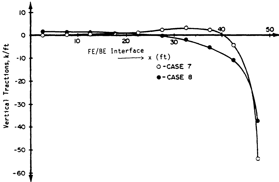
Figure 16b. Vertical tractions at the interface for cases 7 and 8 with concentrated load of 250 k at each end of the beam
