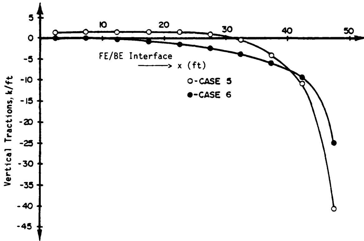
Figure 15b. Vertical tractions at the interface for cases 5 and 6 with concentrated load of 250 k at each end of the beam
