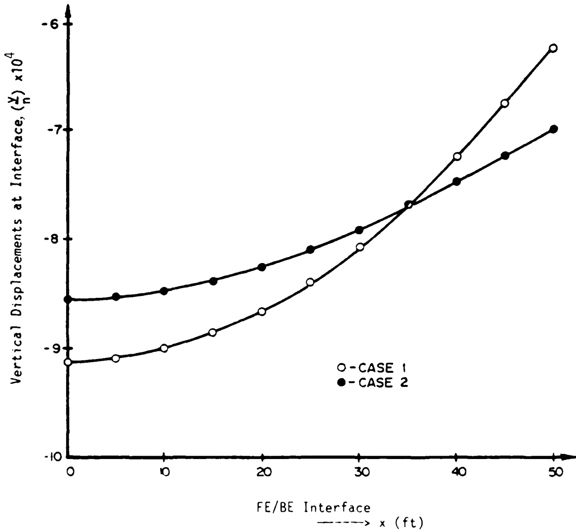
Figure 9a. Vertical displacements at the interface for cases 1 and 2 with uniformly distributed load 5 k/ft on top of beam
