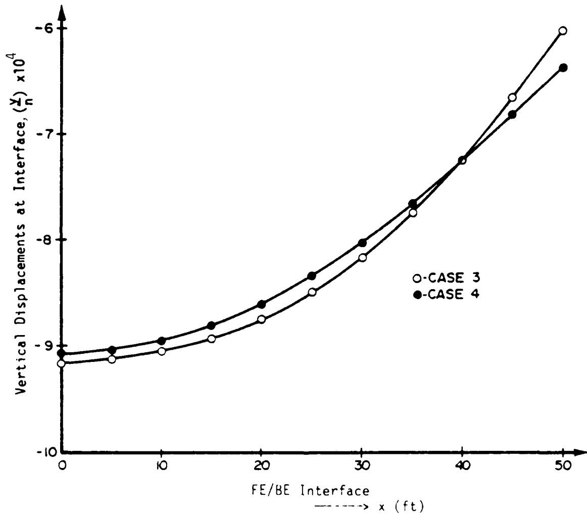
Figure 10a. Vertical displacements at the interface for cases 3 and 4 with uniformly distributed load 5 k/ft on top of beam
