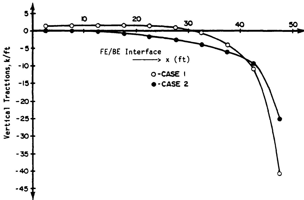
Figure 13b. Vertical tractions at the interface for cases 1 and 2 with concentrated load of 250 k at each end of the beam
