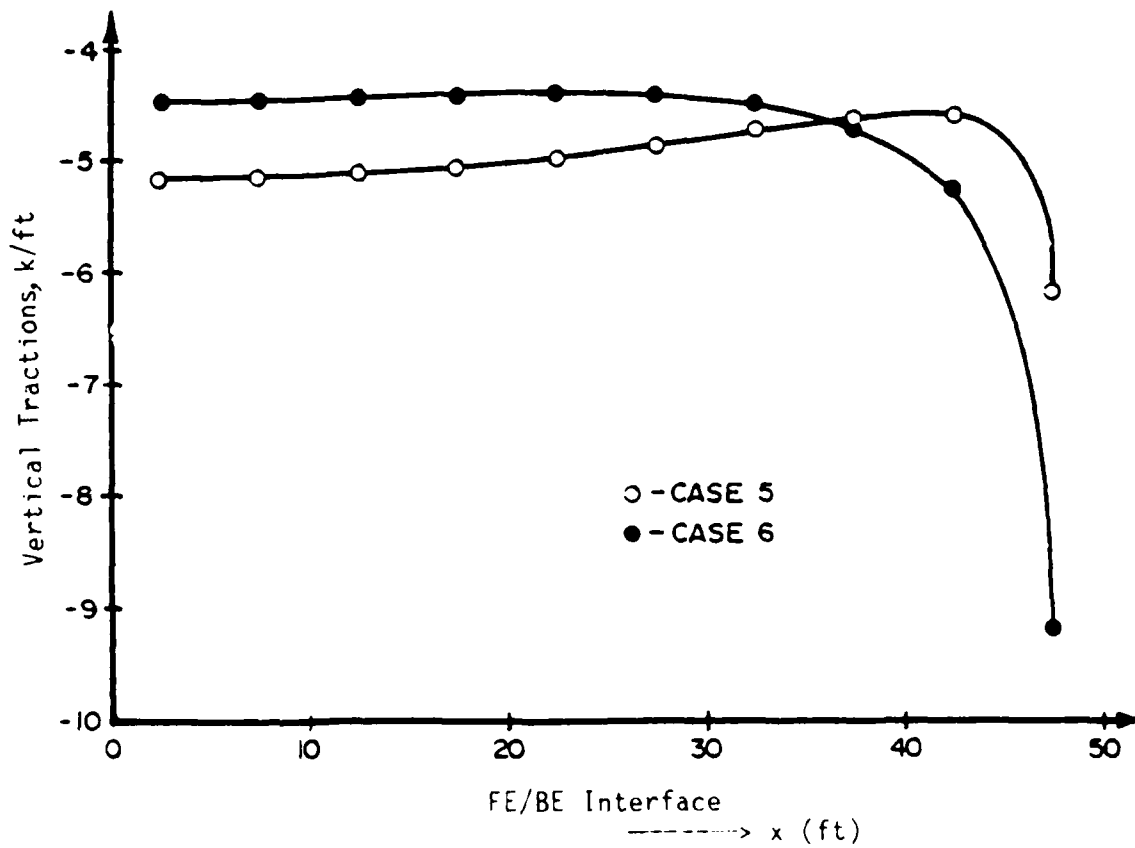
Figure 11b. Vertical tractions at the interface for cases 5 and 6 with uniformly distributed load 5 k/ft on top of beam
