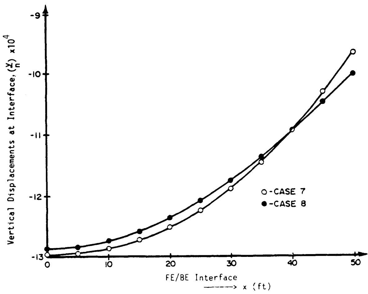
Figure 12a. Vertical displacements at the interface for cases 7 and 8 with uniformly distributed load 5 k/ft on top of beam
