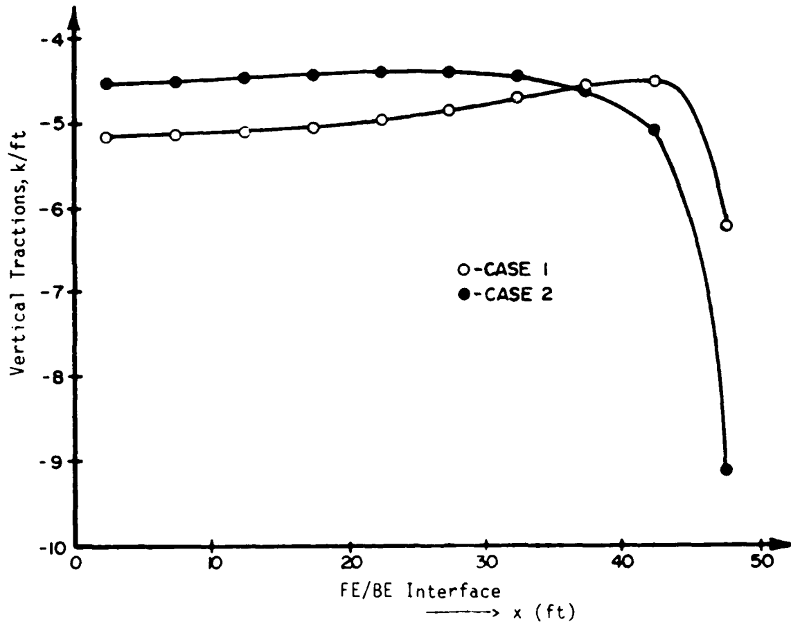
Figure 9b. Vertical tractions at the interface for cases 1 and 2 with uniformly distributed load 5 k/ft on top of beam
