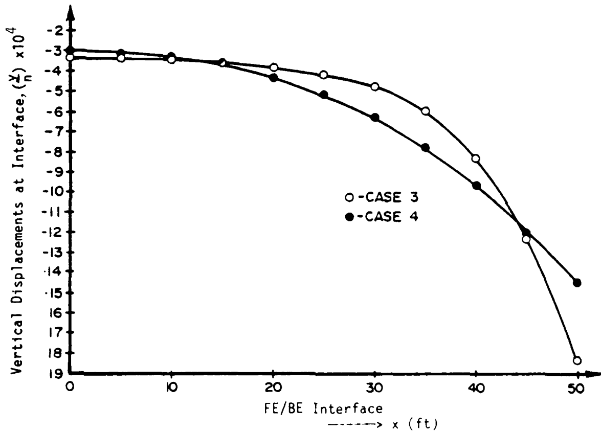
Figure 14a. Vertical displacements at the interface for cases 3 and 4 with concentrated load of 250 k at each end of the beam
