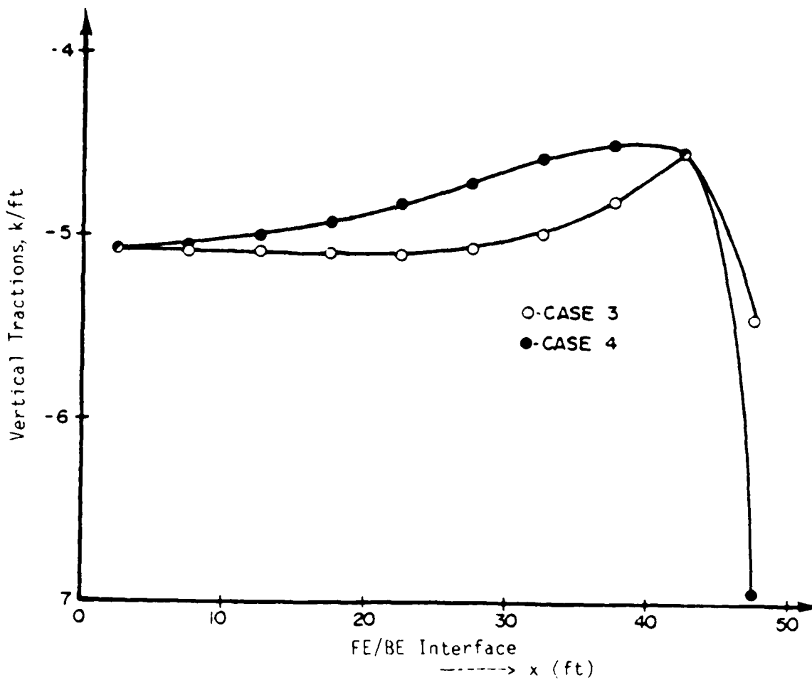
Figure 10b. Vertical tractions at the interface for cases 3 and 4 with uniformly distributed load 5 k/ft on top of beam
