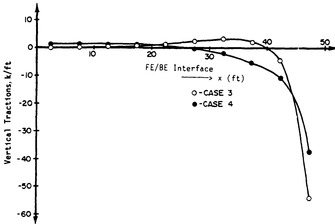
Figure 14b. Vertical tractions at the interface for cases 3 and 4 with concentrated load of 250 k at each end of the beam
