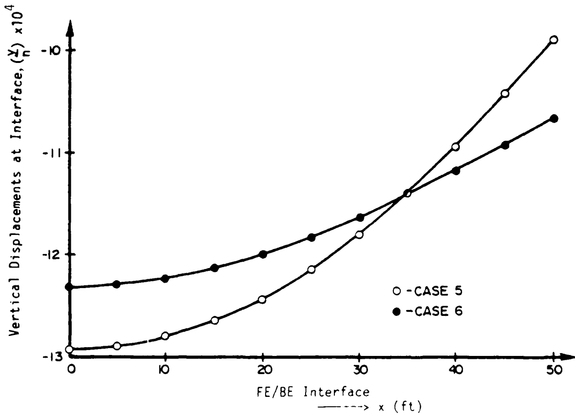
Figure 11a. Vertical displacements at the interface for cases 5 and 6 with uniformly distributed load 5 k/ft on top of beam
