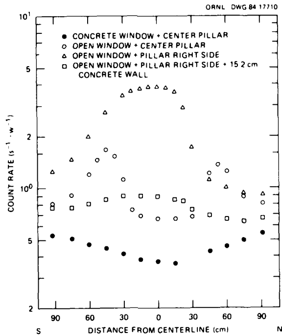
Fig. 16. Count rate profiles for 5-in. Bonner ball along horizontal traverses 61 cm in front of rear wall of block house (Items II A, B, C, D).
