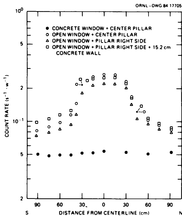
Fig. 11. Count rate profiles for Cd-covered BF_3 counter along horizontal traverses 61 cm beyond front wall of block house (Items II A, B, C, D).
