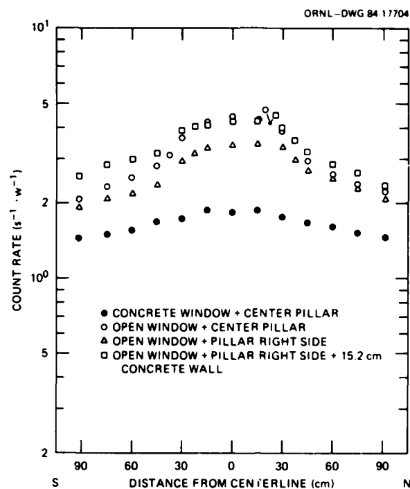
Fig. 10. Count rate profiles for bare BF_3 counter along horizontal traverses 61 cm beyond front wall of block house (Items II A, B, C, D).
