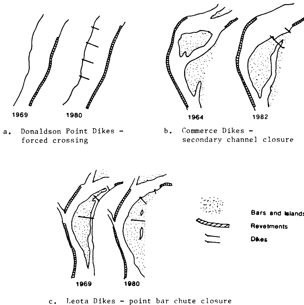
Figure 1. Dike field types
