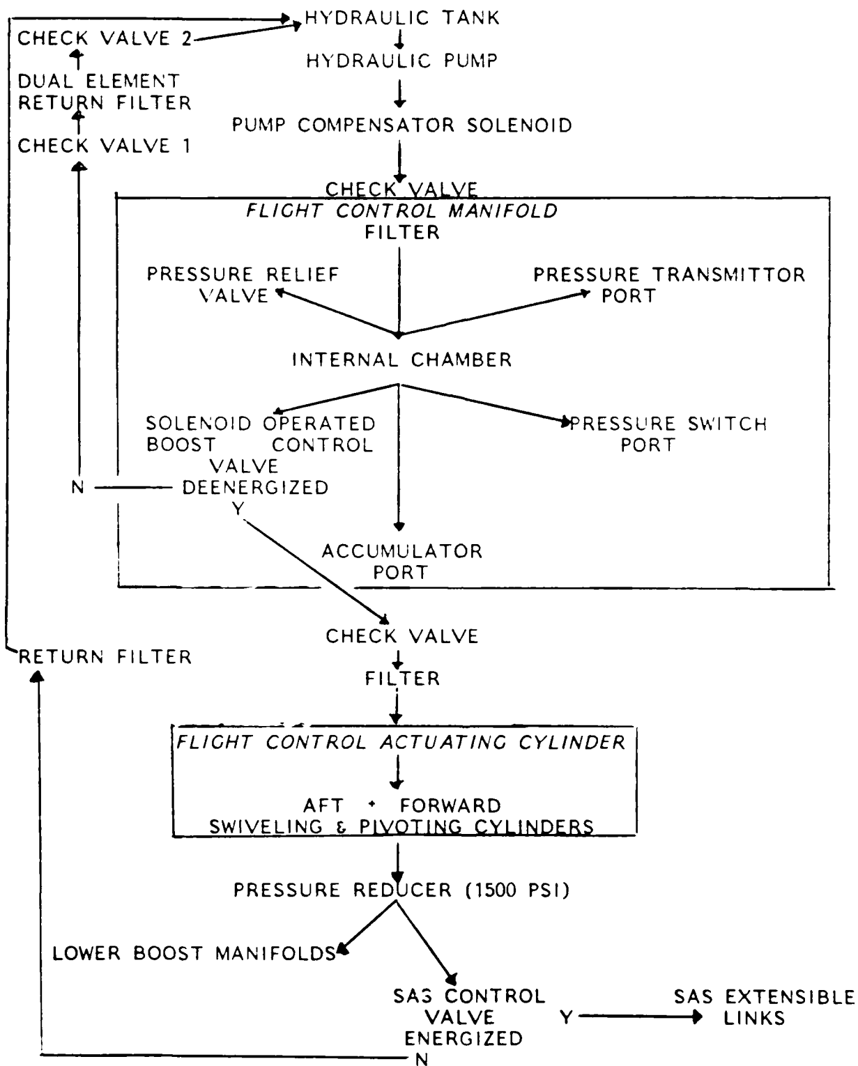
HYDRAULIC FLIGHT CONTROL SYSTEM OPERATION FIGURE 5
