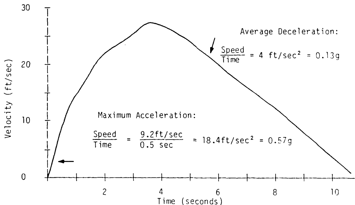
Figure 4. Typical Acceleration/Deceleration Curve.
