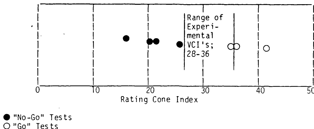
Figure 2. Example of Graphic Determination of Experimental VCI.
