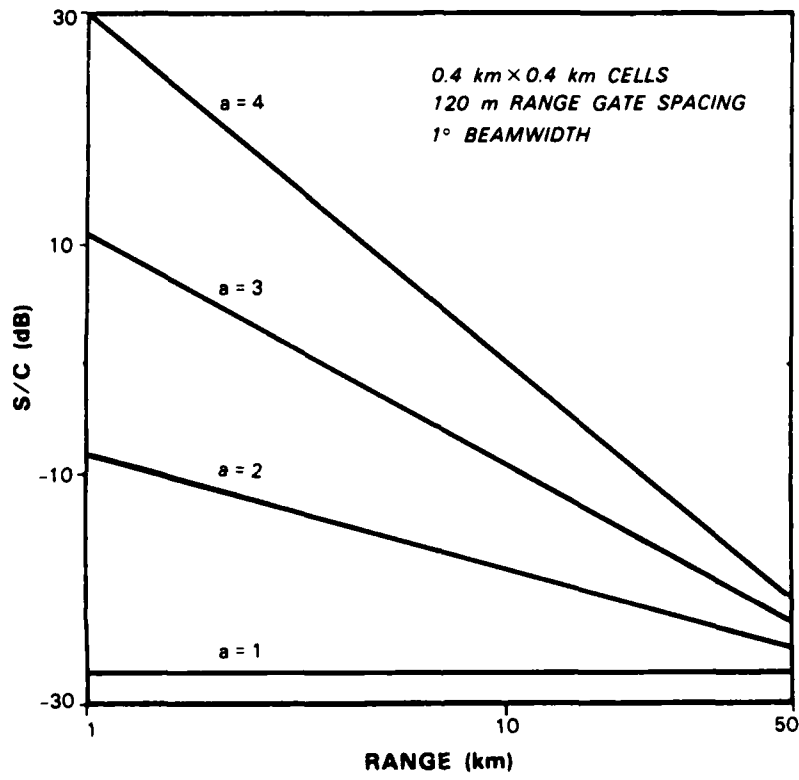
Figure IV-6. SCR vs range after CMAP filter for 0 dBz signal, radar-cross-section density, and representative Weibull slopes.
