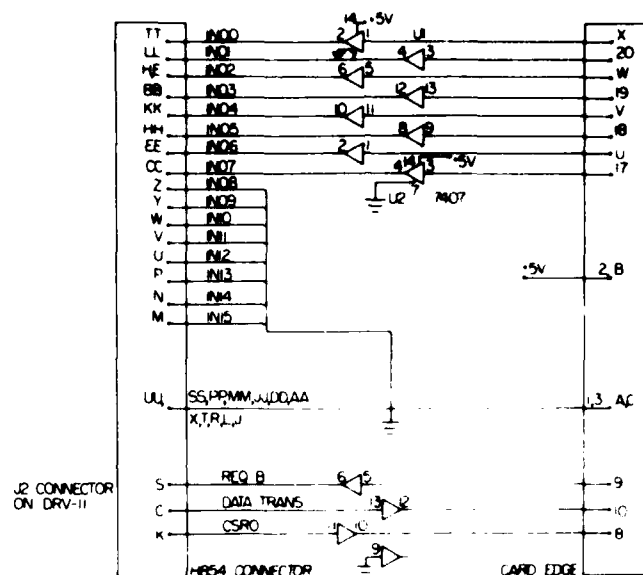
Figure 11. Schematic of Line Current Driver Interface Board
