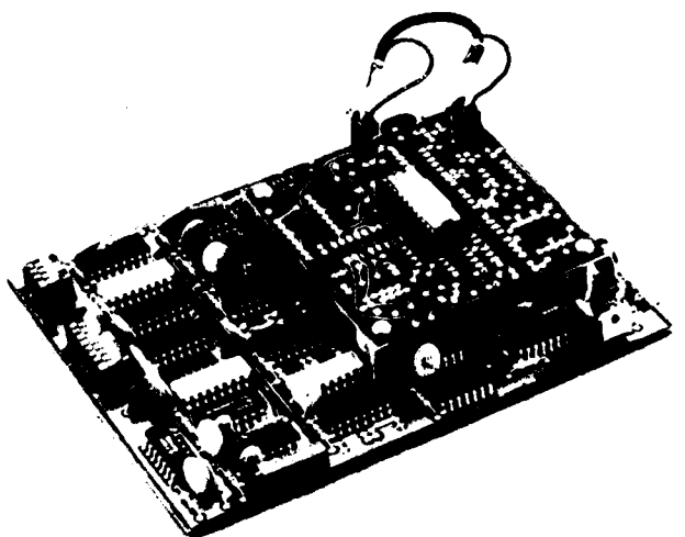
Figure 5. Photograph of RC702A Satellite Board With CCPD 256-Photodiode Array Attached to the RC700A Motherboard
