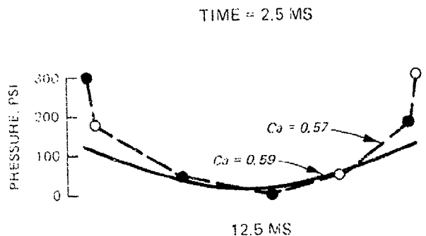
Figure 4.4. Actual and theoretical pressure distributions for Test YE3.
