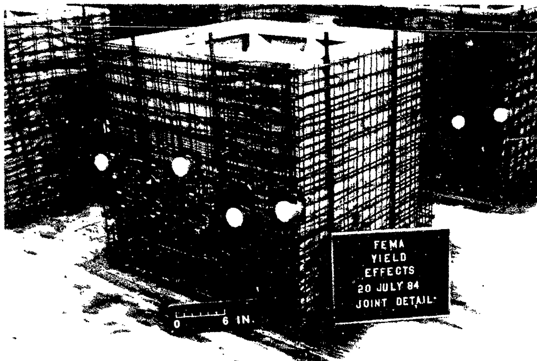
Figure 2.2. Yield effects tests, typical joint detail.
