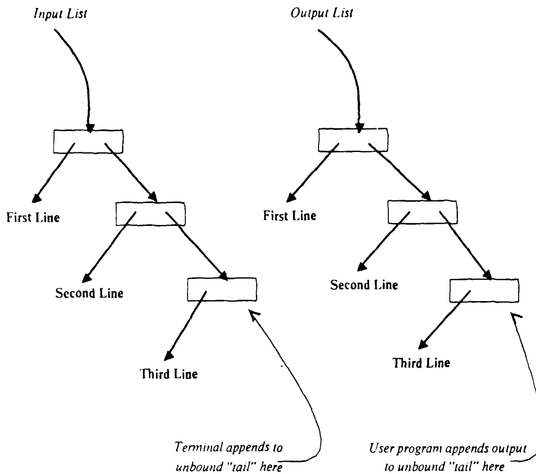
Figure 2-15: Terminal input/output on streams with "unbound tails".
