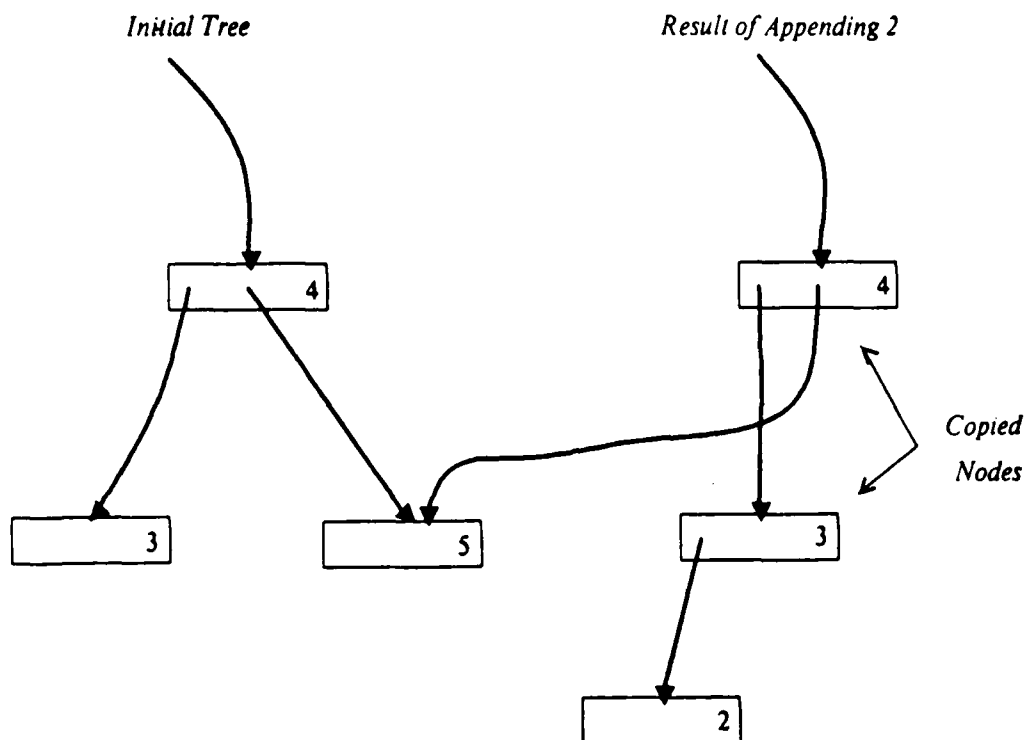
Figure 1-1: An integer being appended to a tree in the tree-append program.
