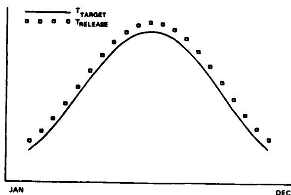
Figure 3. Release temperatures with long-term operational strategy
