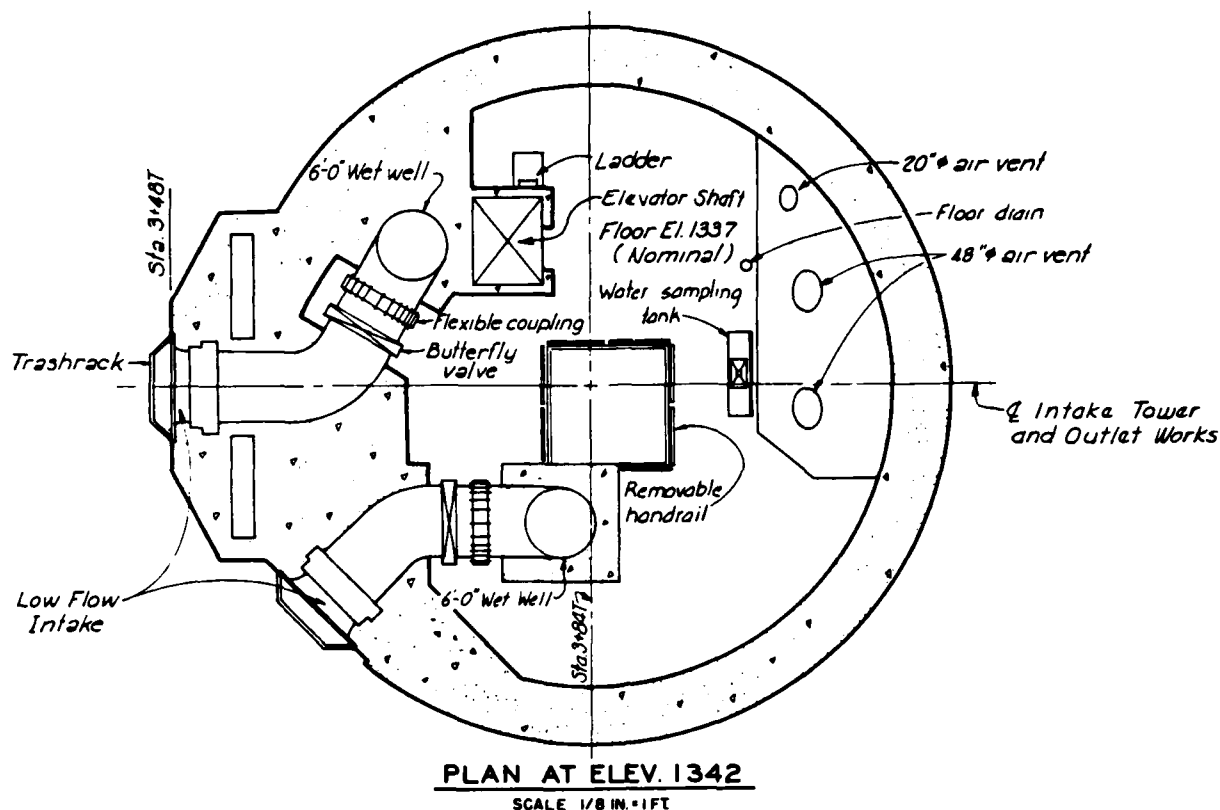
Figure 2. Bloomington Lake Intake Control Tower
