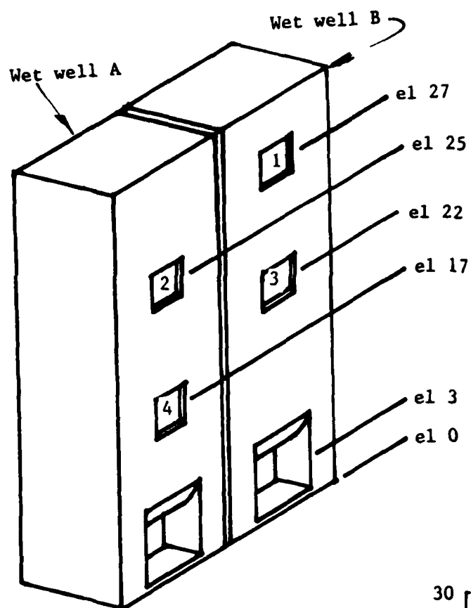
FIG. 1.--Structure schematic
