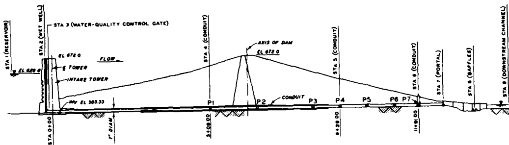
Fig. 2. Beltzville Dam Water Quality Measurement Stations
