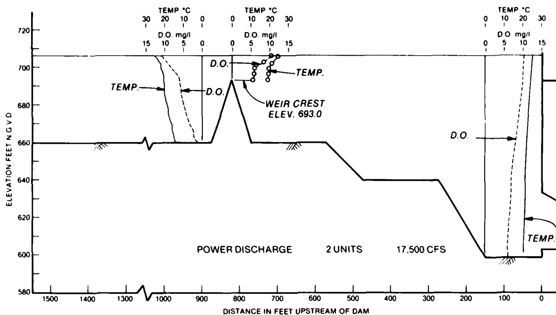
Figure 3 - Temperature and Dissolved Oxygen Profiles With Two Power Units in Operation
