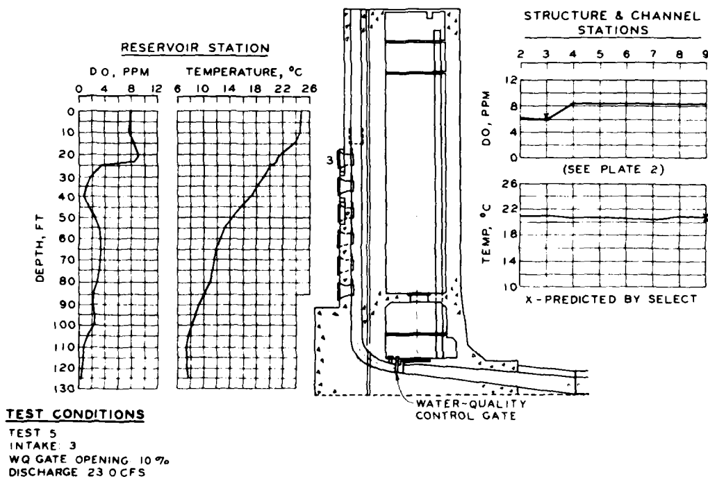
Fig. 3. Beltzville Dam Water Quality Measurements
