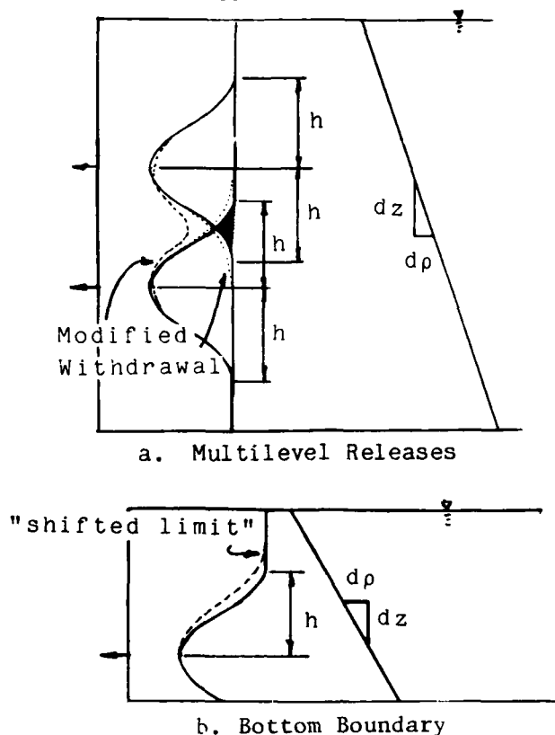
Figure 3. Withdrawal Zone Interference
