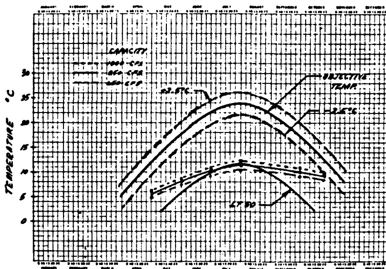
Figure 1. Expected downstream temperature with 3 capacities when the maximum reasonable discharge of 4000 cfs is released from Cowanesque Lake.
