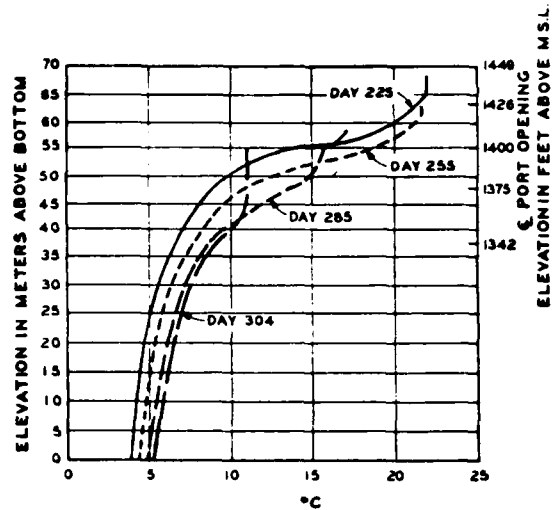
C. COMPUTED STRATIFICATION BREAKDOWN
