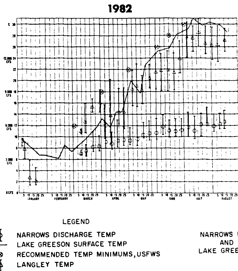
FIGURE 3. INFLOW, LAKE AND DISCHARGE TEMPERATURE TO LAKE GREESON
