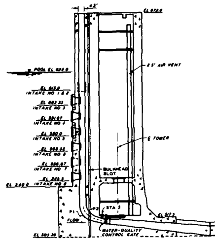
Fig. 1. Beltzville Dam Intake Tower
