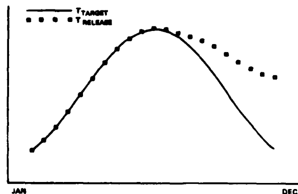
Figure 1. Release temperature with day-to-day operational strategy.
