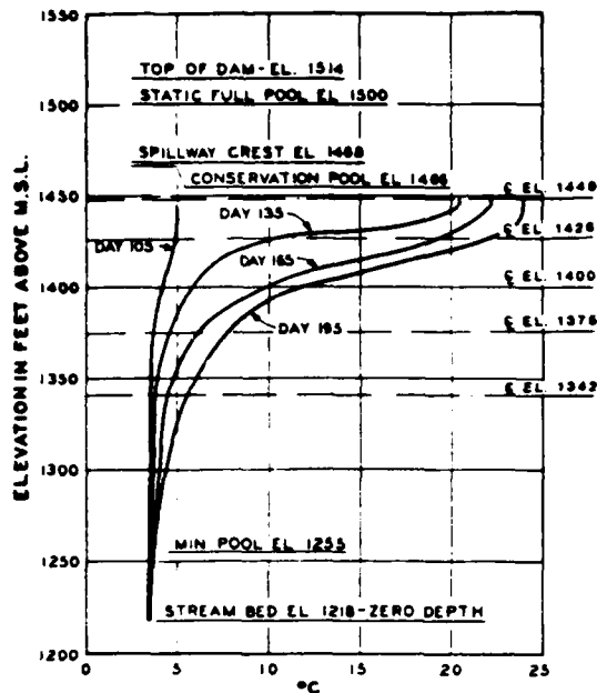
B. COMPUTED STRATIFICATION BUILD-UP
