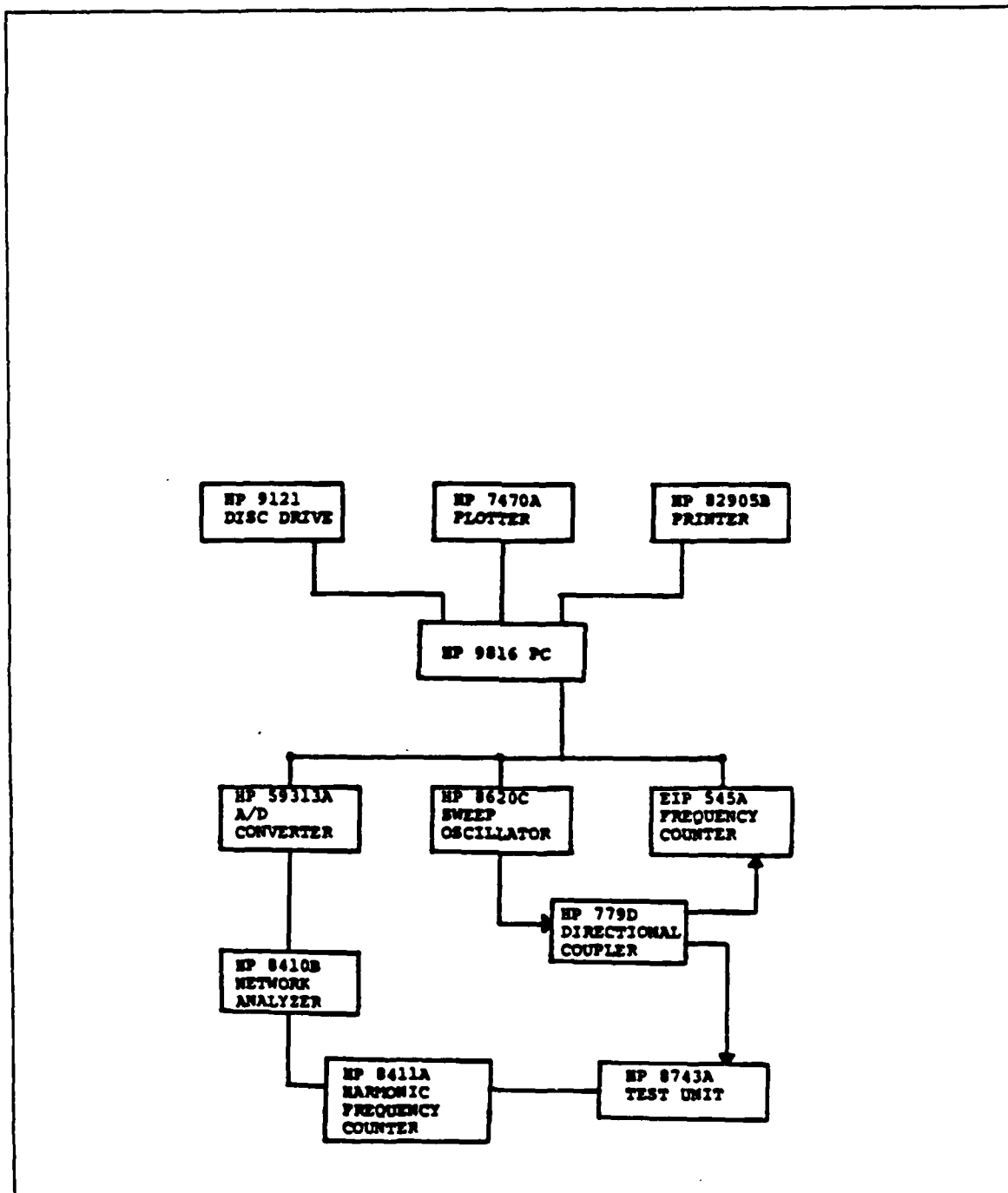
Figure B.3: Block diagram for automated data collection system
