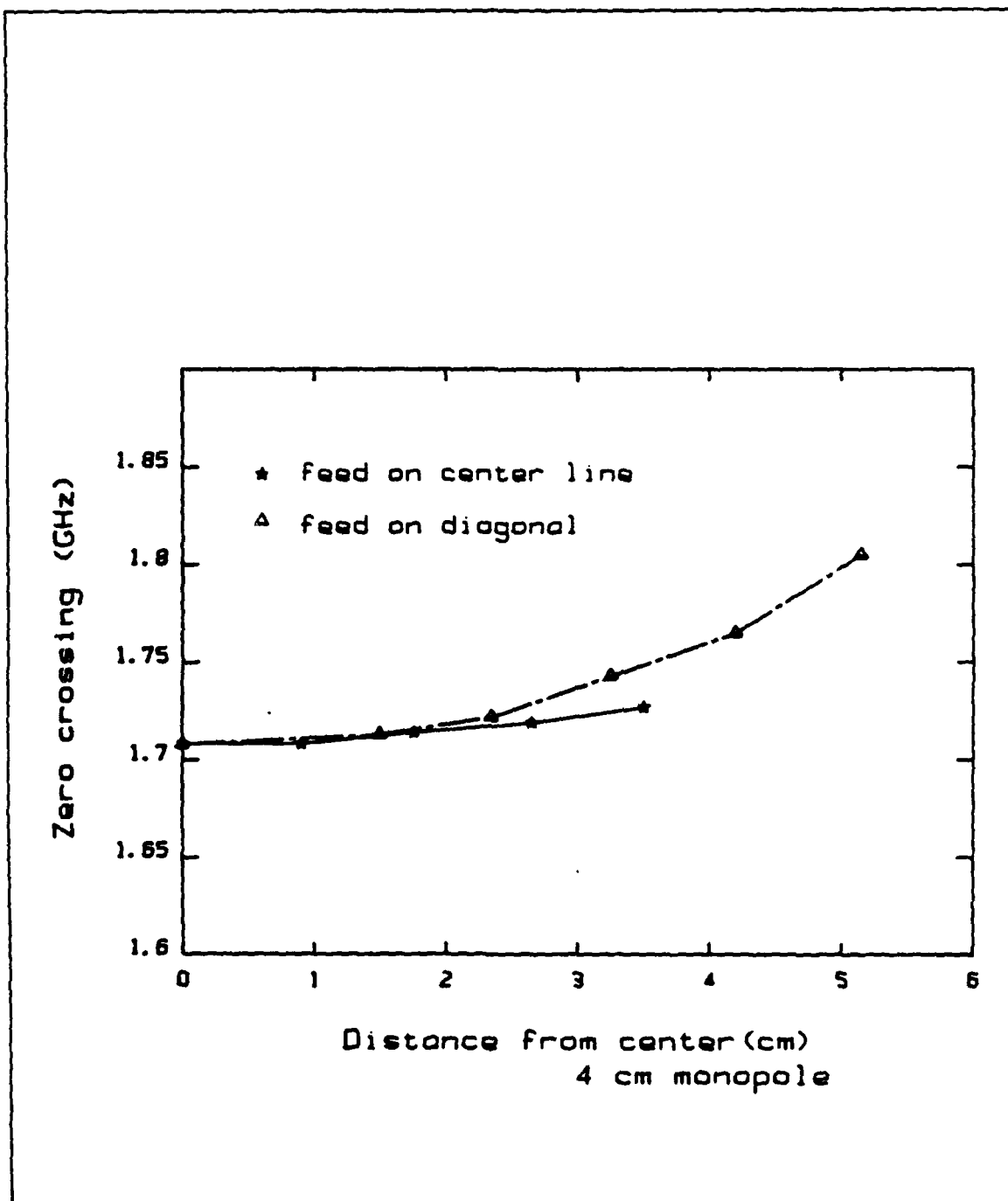
Figure C.23: Zero crossing frequency versus distance from center; 4 cm monopole
