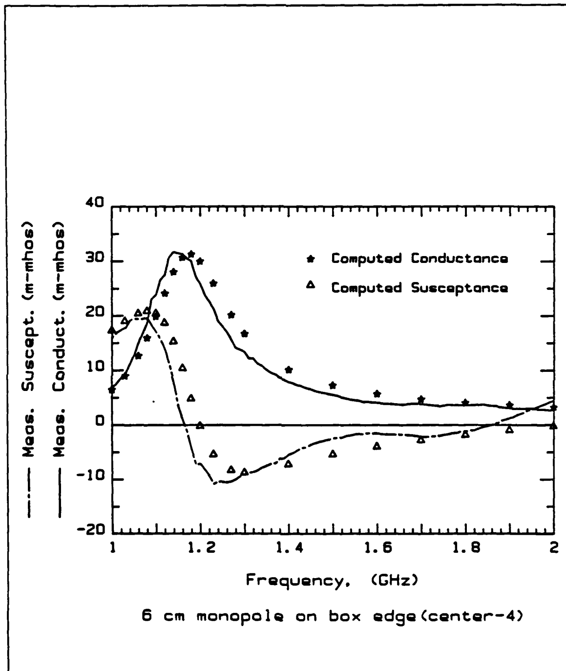
Figure D.5: 6 cm Monopole at box edge(center-4)
