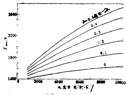
Fig.3. The maximum allowed gas temperature vs the thickness of ceramic coating and the internal cooling intensity. (1: Kcal/m^2 hr; 2: mm)
