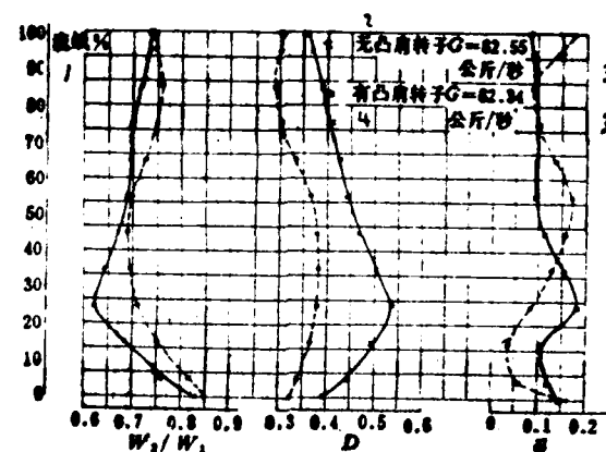
Fig. 6(a) Radial distribution of flow parameters at the outlet of rotor. (1: flow line; 2: rotor without part span shroud; 3: Kg/sec; 4: rotor with part span shroud)
