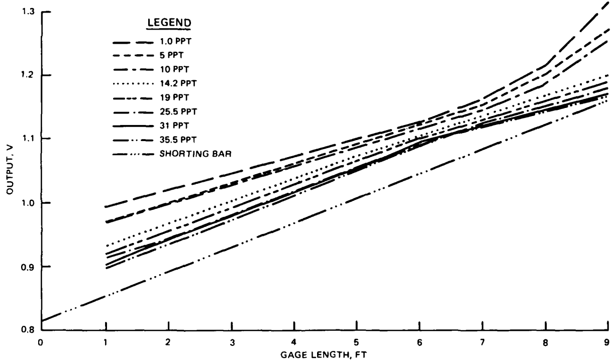
Figure 8. Variation in gage linearity as a function of salinity
